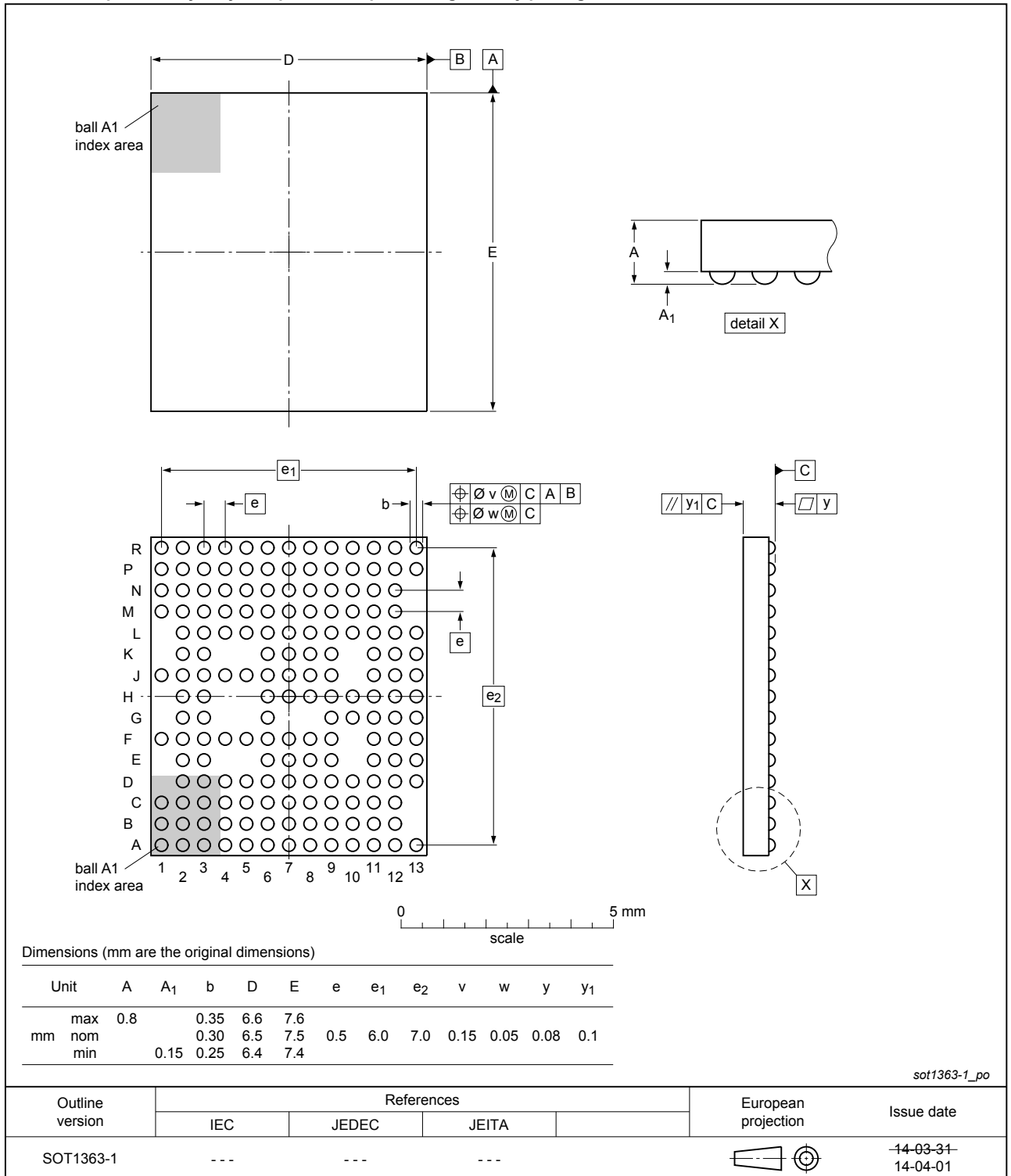
Fig. 1. Package outline WFBGA171 (SOT1363-1)
