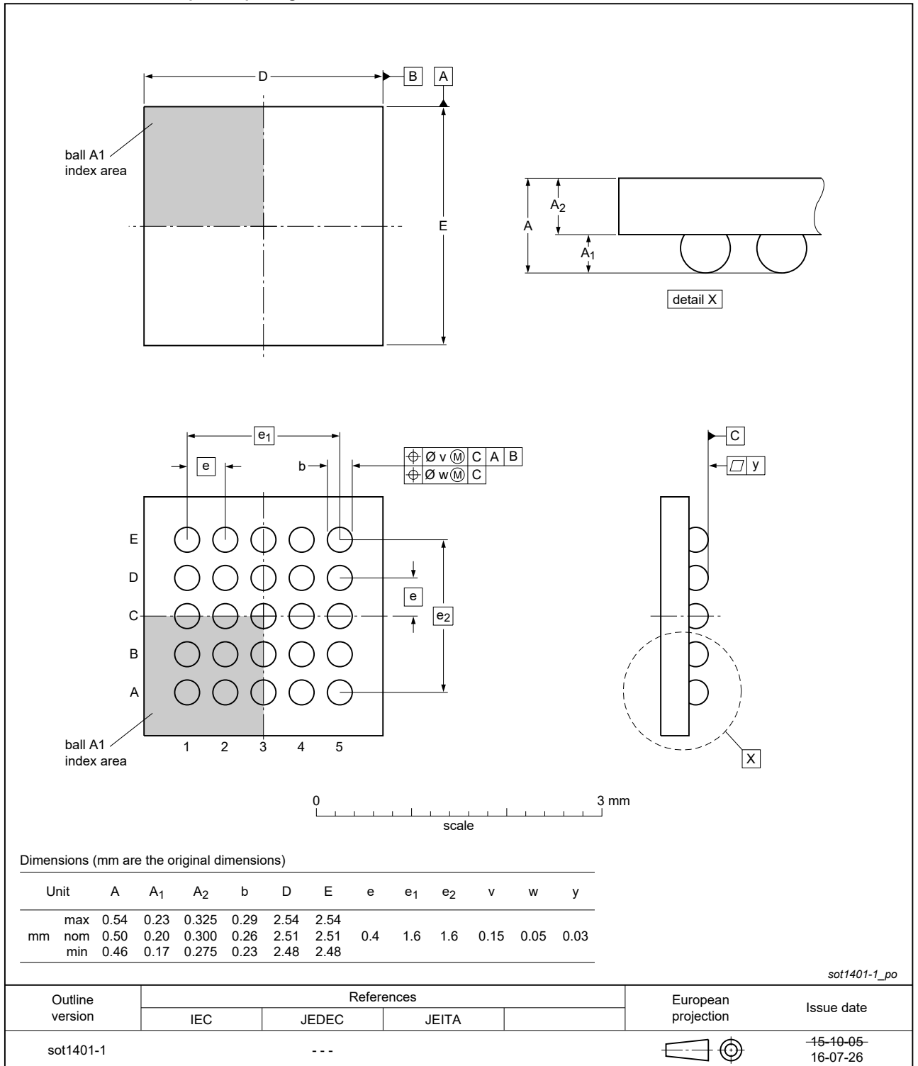
Fig. 1. Package outline WLCSP25 (SOT1401-1)
