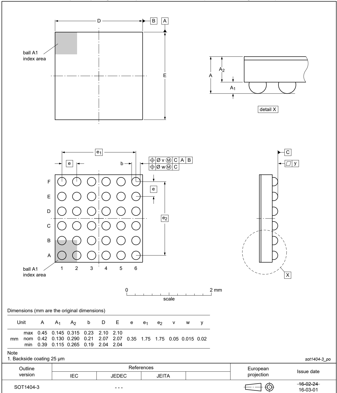
Fig. 1. Package outline WLCSP36 (SOT1404-3)
