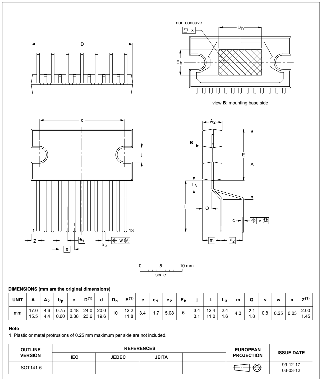
Fig. 1. Package outline DBS13P (SOT141-6)
