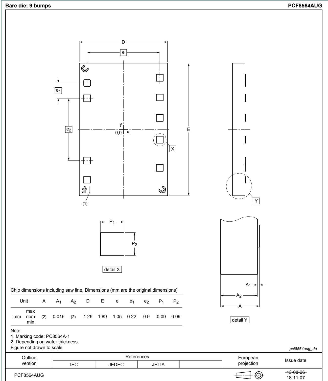
Figure 1. Package outline WLCSP9 (SOT1425-2)
