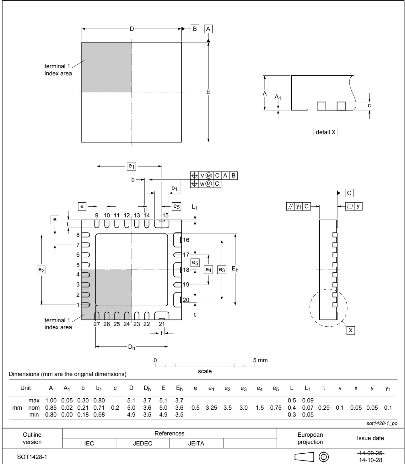
Fig. 1. Package outline HVQFN27 (SOT1428-1)
