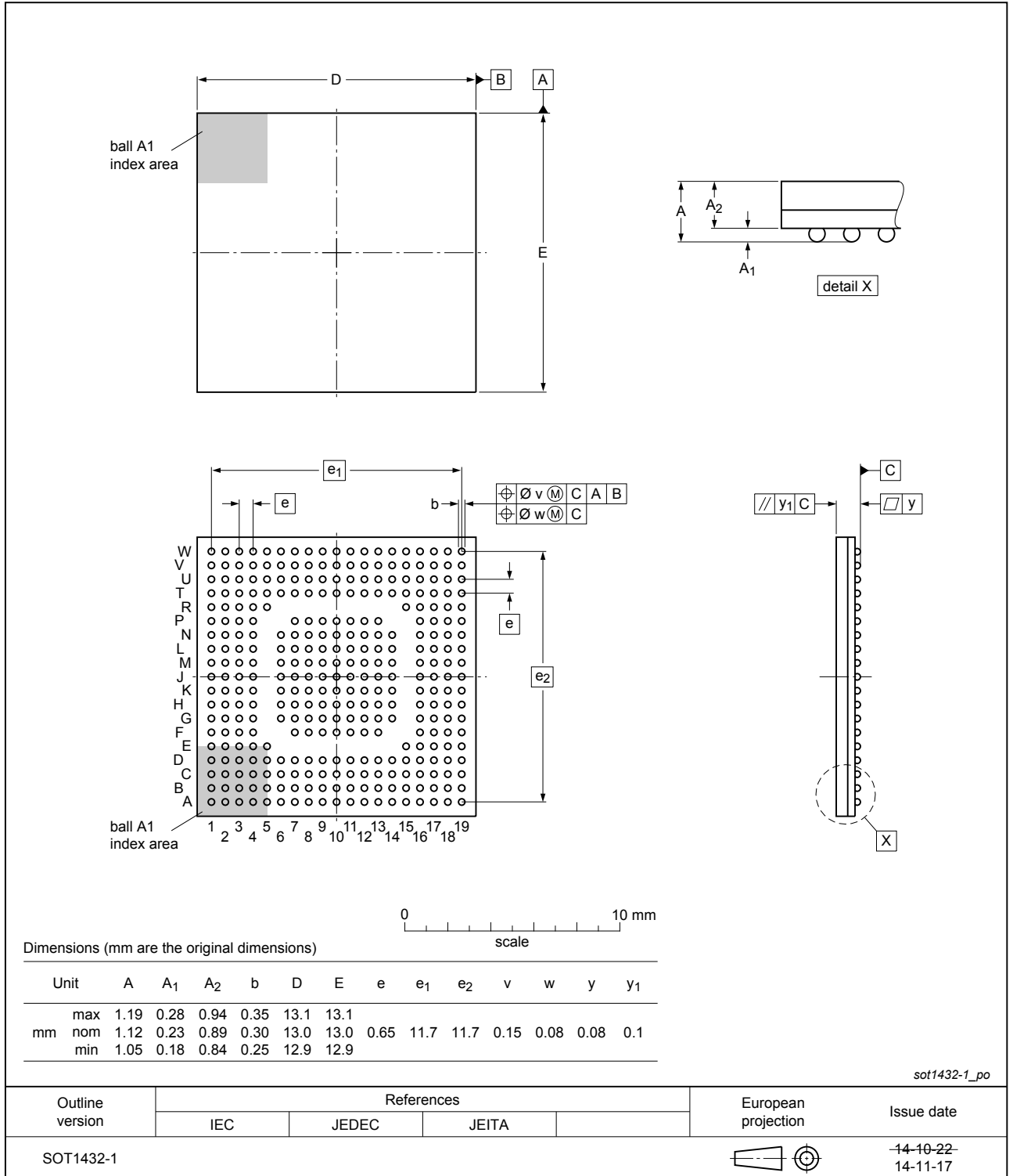
Fig. 1. Package outline TFBGA321 (SOT1432-1)
