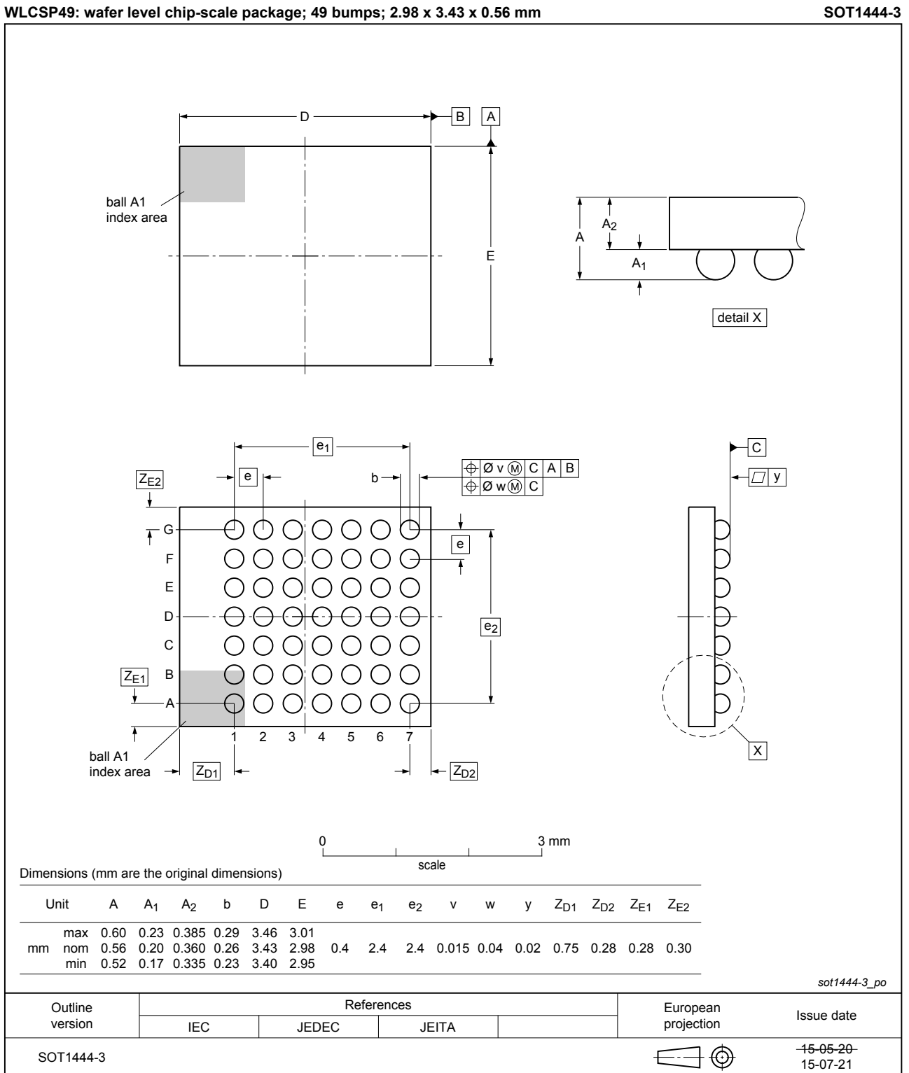
Fig. 1. Package outline WLCSP49 (SOT1444-3)
