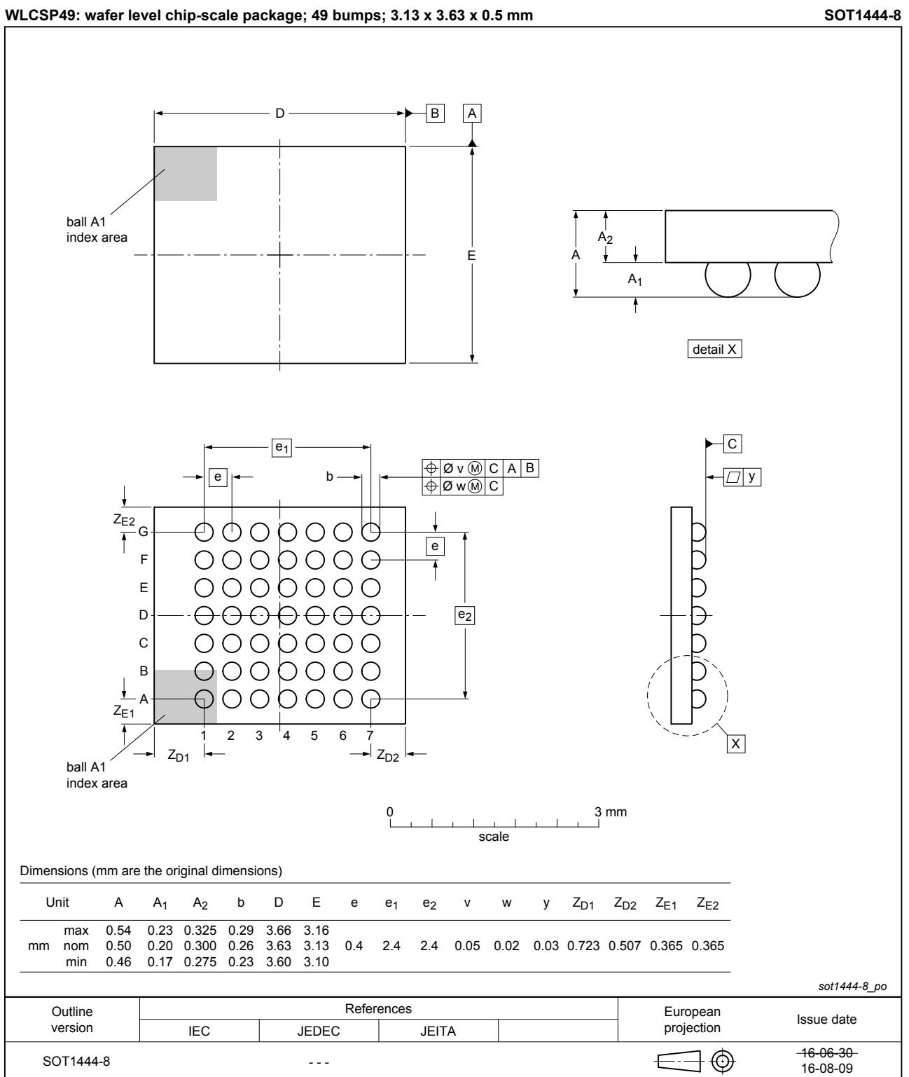
Fig. 1. Package outline WL CSP (SOT1444-8)
