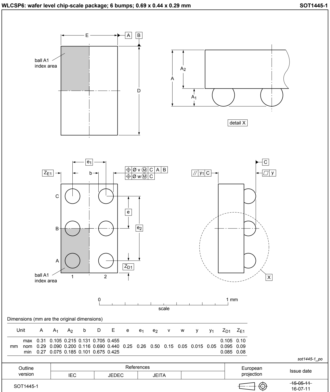
Fig. 1. Package outline WLCSP6 (SOT1445-1)
