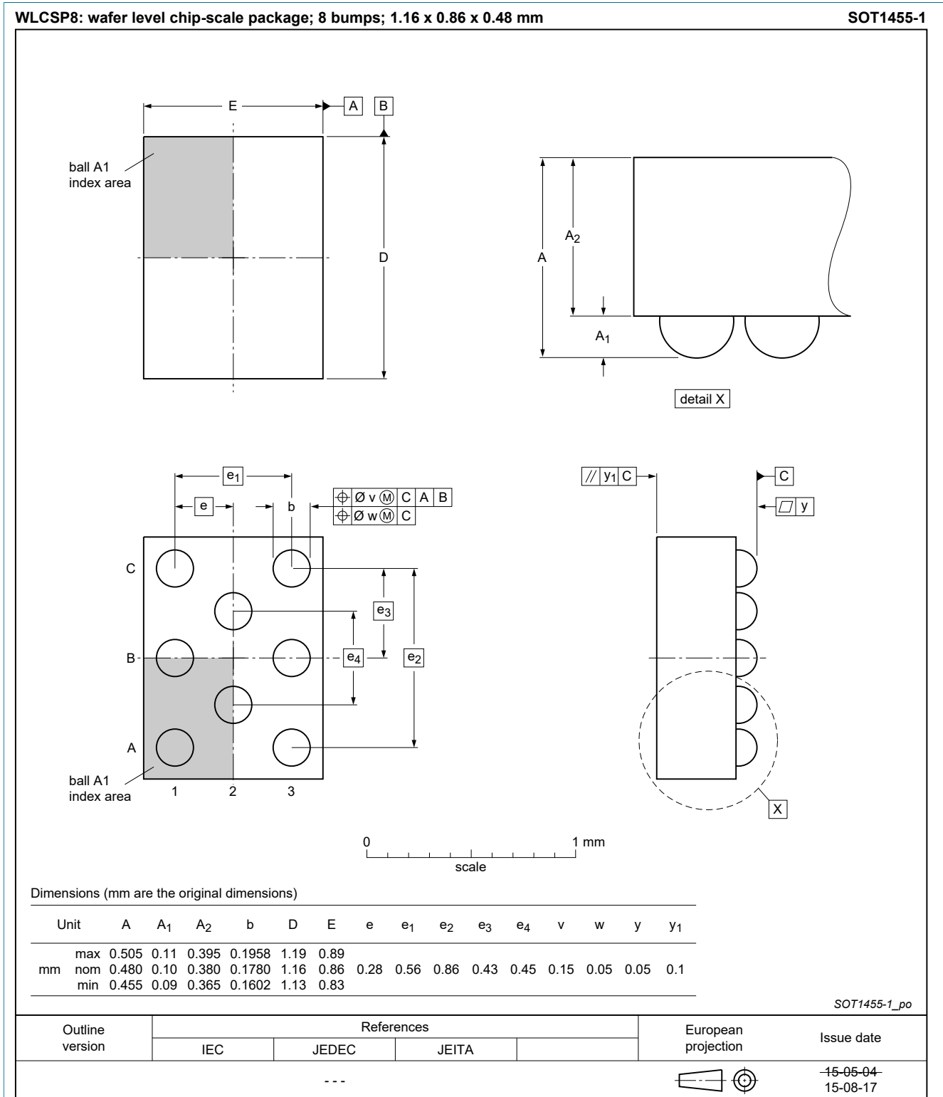
Figure 1. Package outline WLCSP8 (SOT1455-1)
