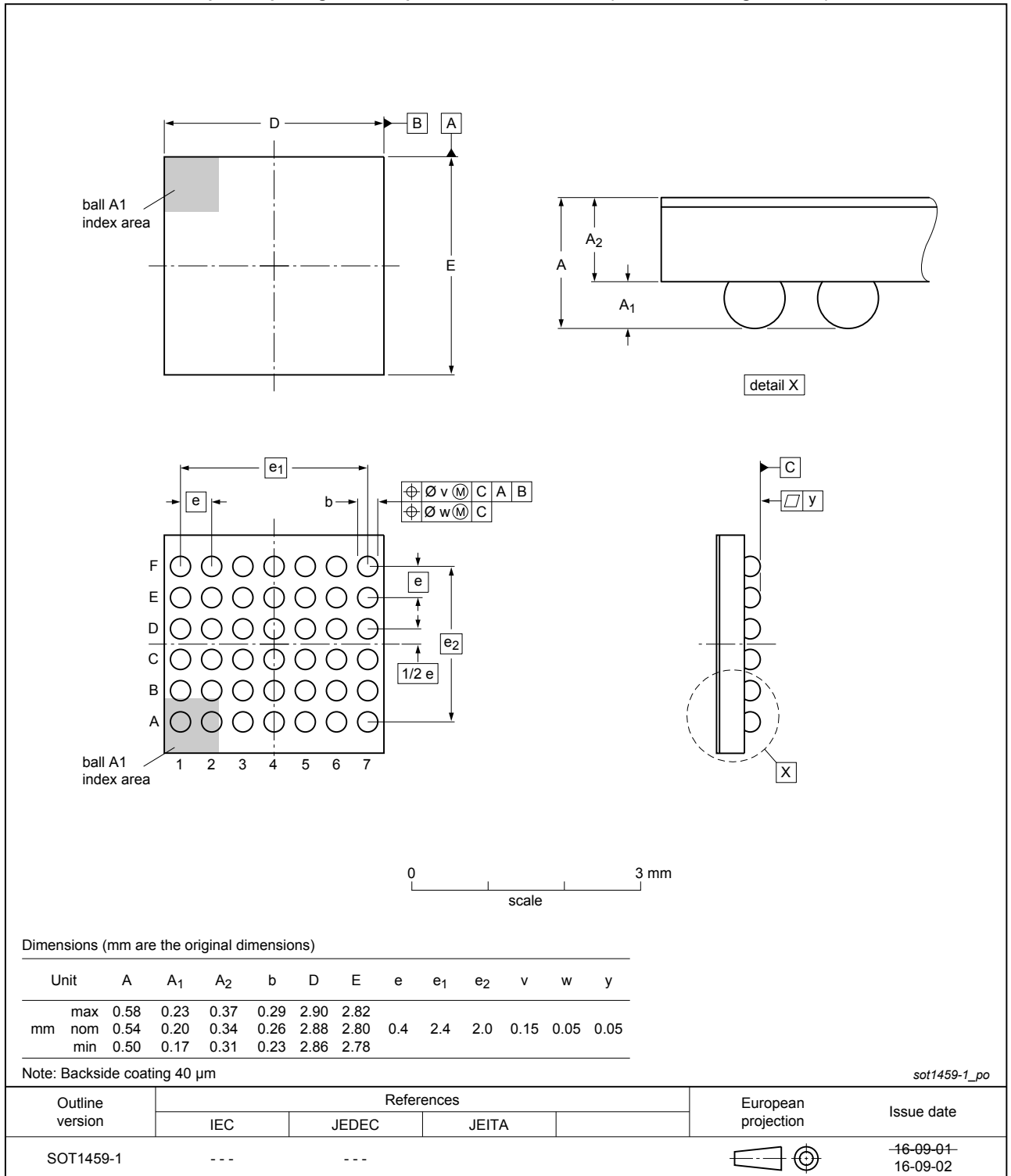
Fig. 1. Package outline WLCSP (SOT1459-1)
