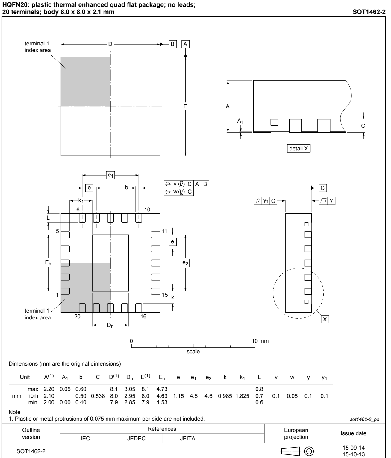
Fig. 1. Package outline HQFN20 (SOT1462-2)
