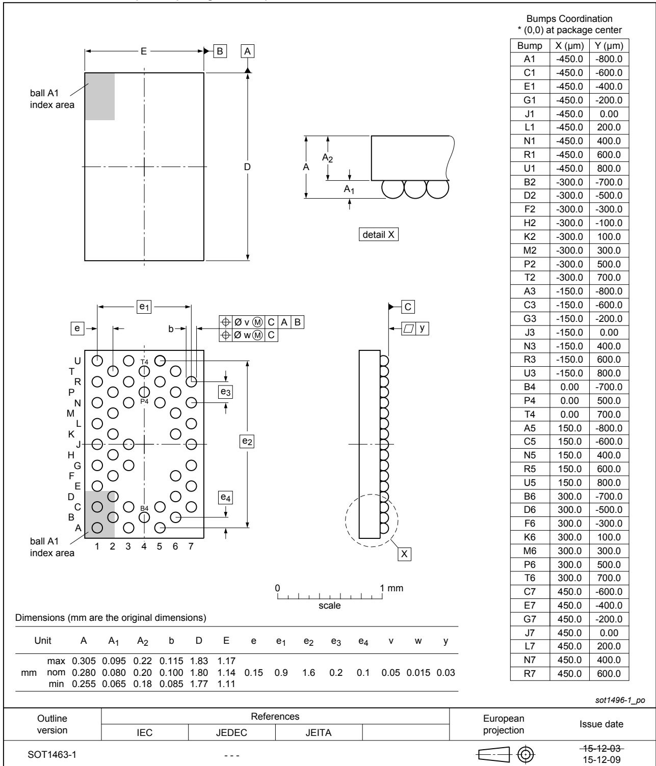
Fig. 1. Package outline WLSCP46 (SOT1463-1)
