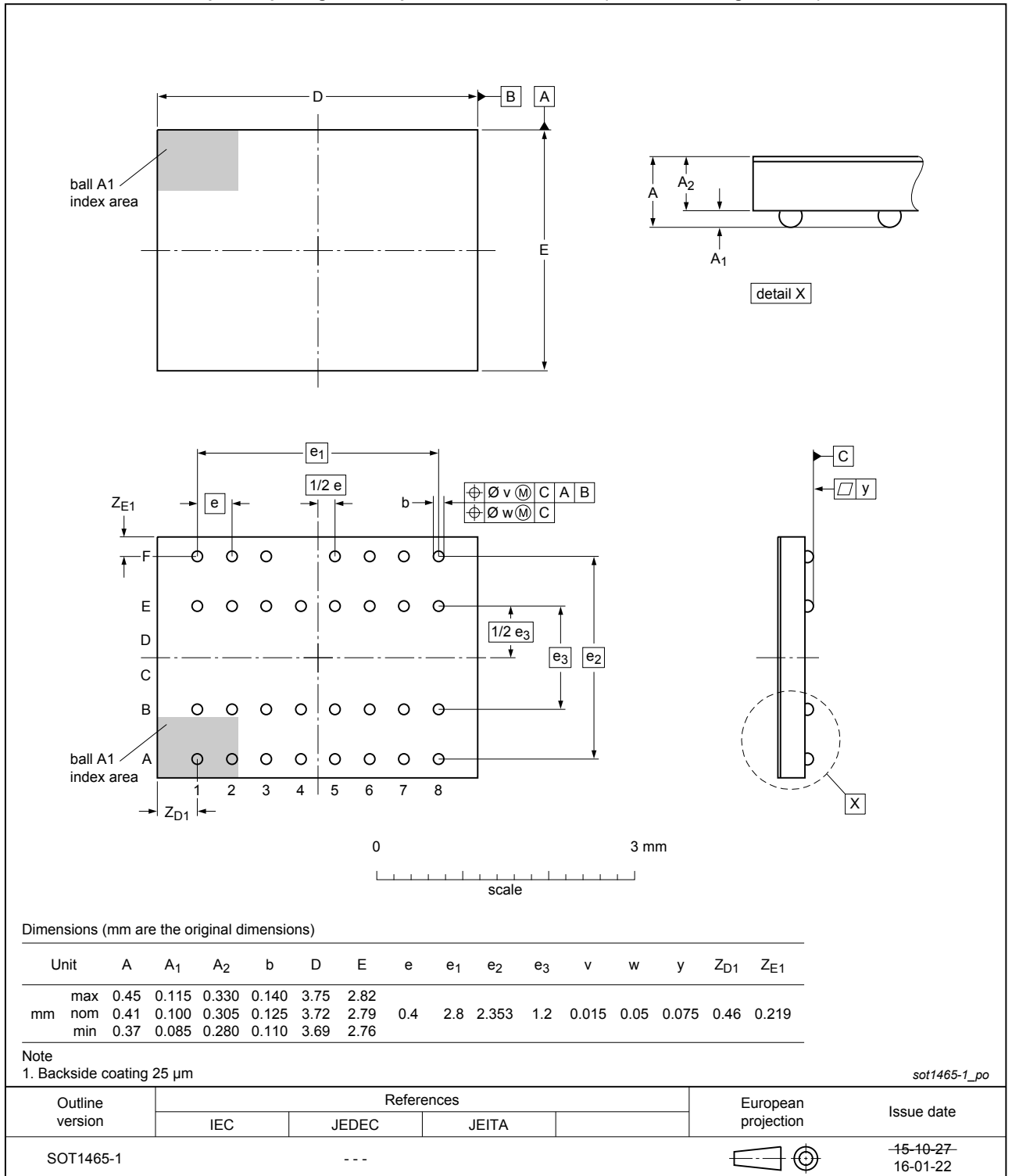
Fig. 1. Package outline WLCSP31 (SOT1465-1)
