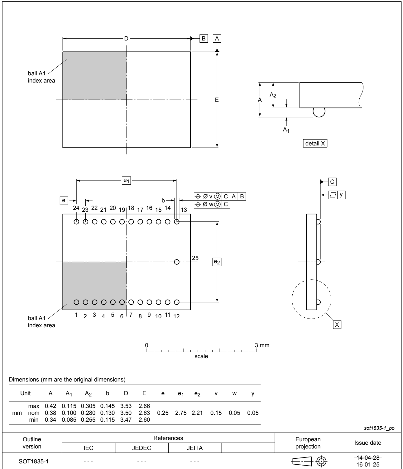
Fig. 1. Package outline WLCSP25 (SOT1835-1)
