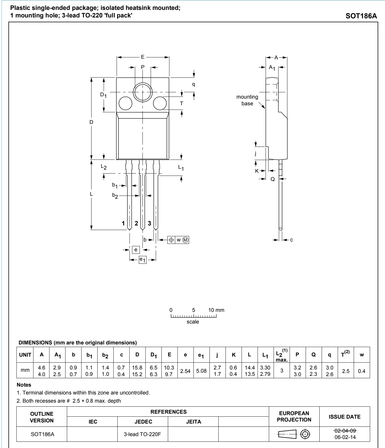
Fig. 1. Package outline TO-220F (SOT186A)
