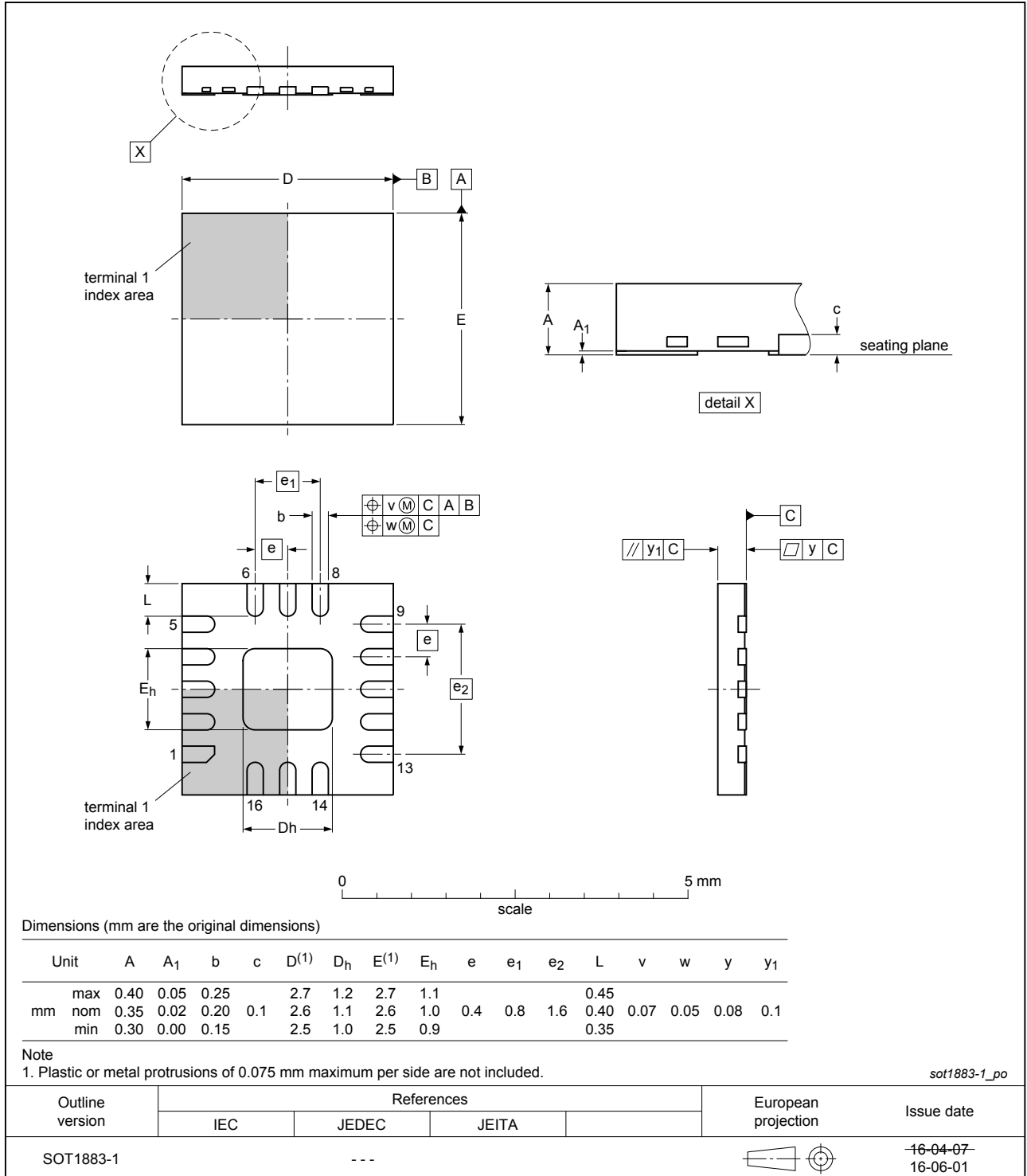
Fig. 1. Package outline HX2QFN (SOT1883-1)
