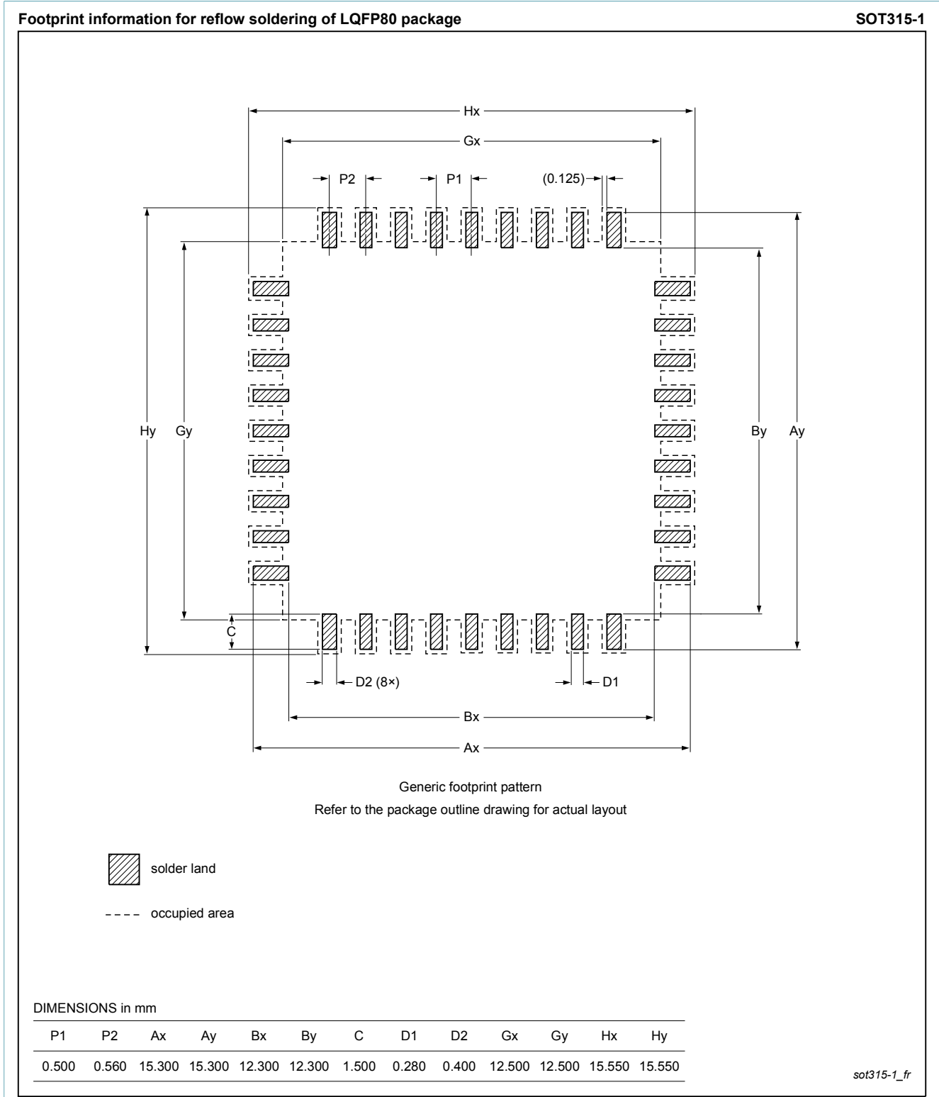
Fig. 2. Reflow soldering footprint for LQFP80 (SOT315-1)
