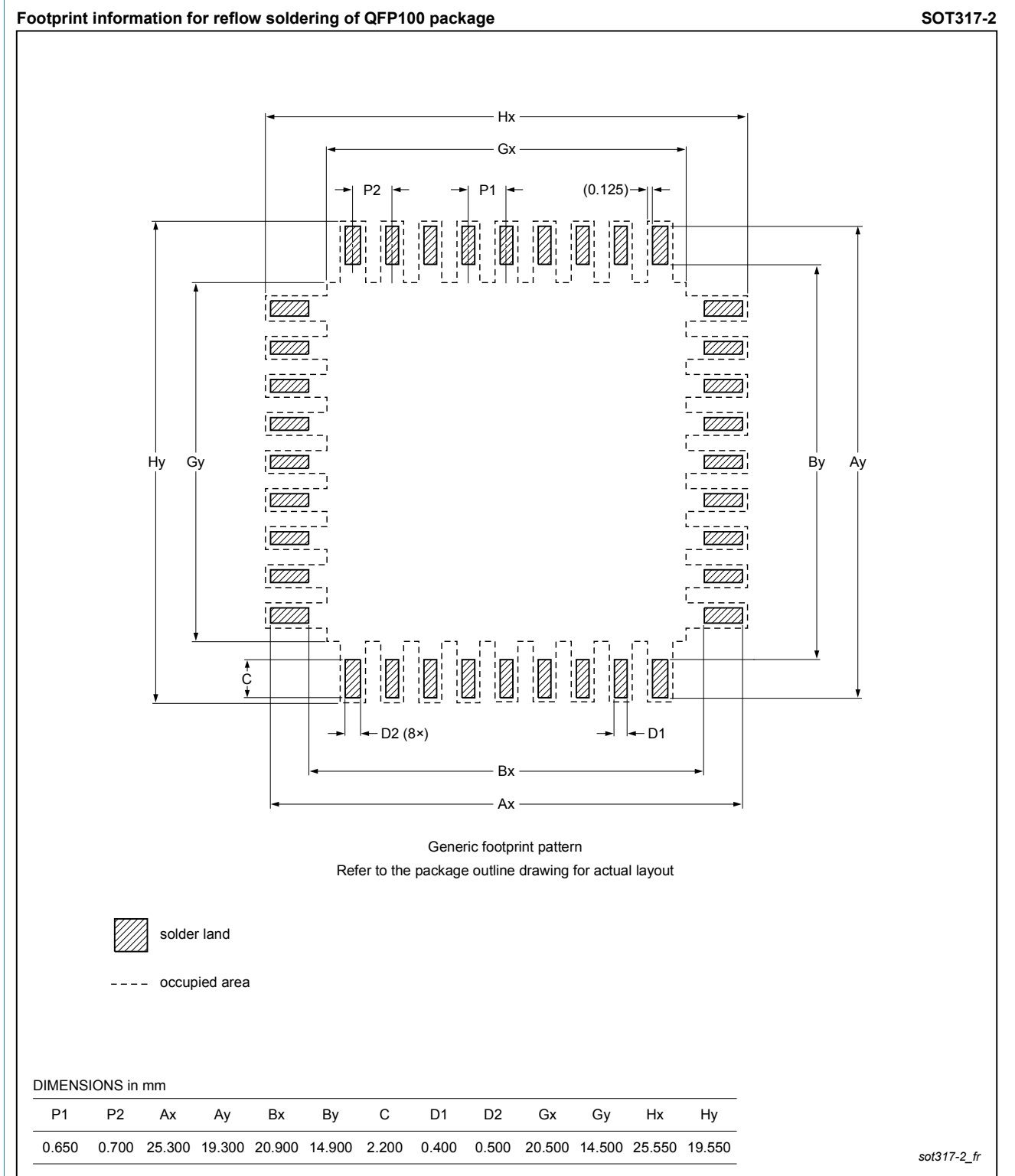
Figure 2. Reflow soldering footprint for QFP100 (SOT317-2)
