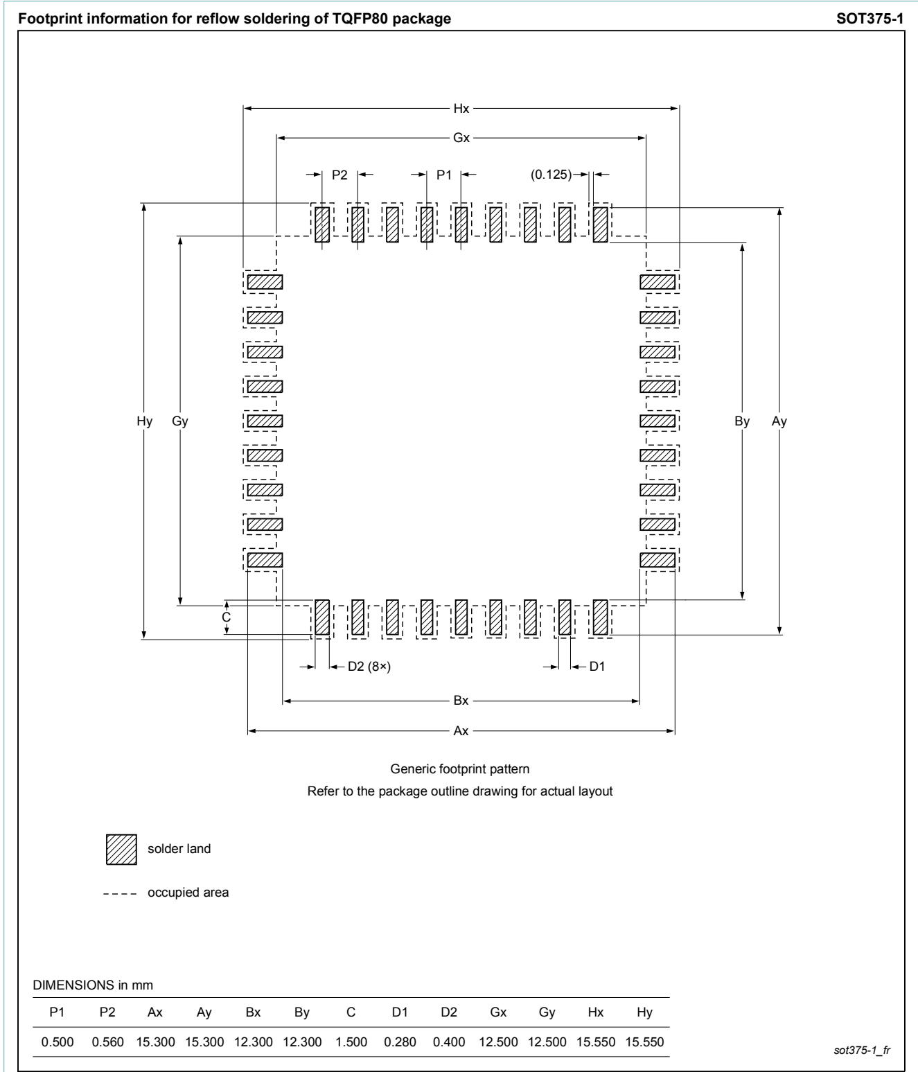
Fig. 2. Reflow soldering footprint for TQFP80 (SOT375-1)
