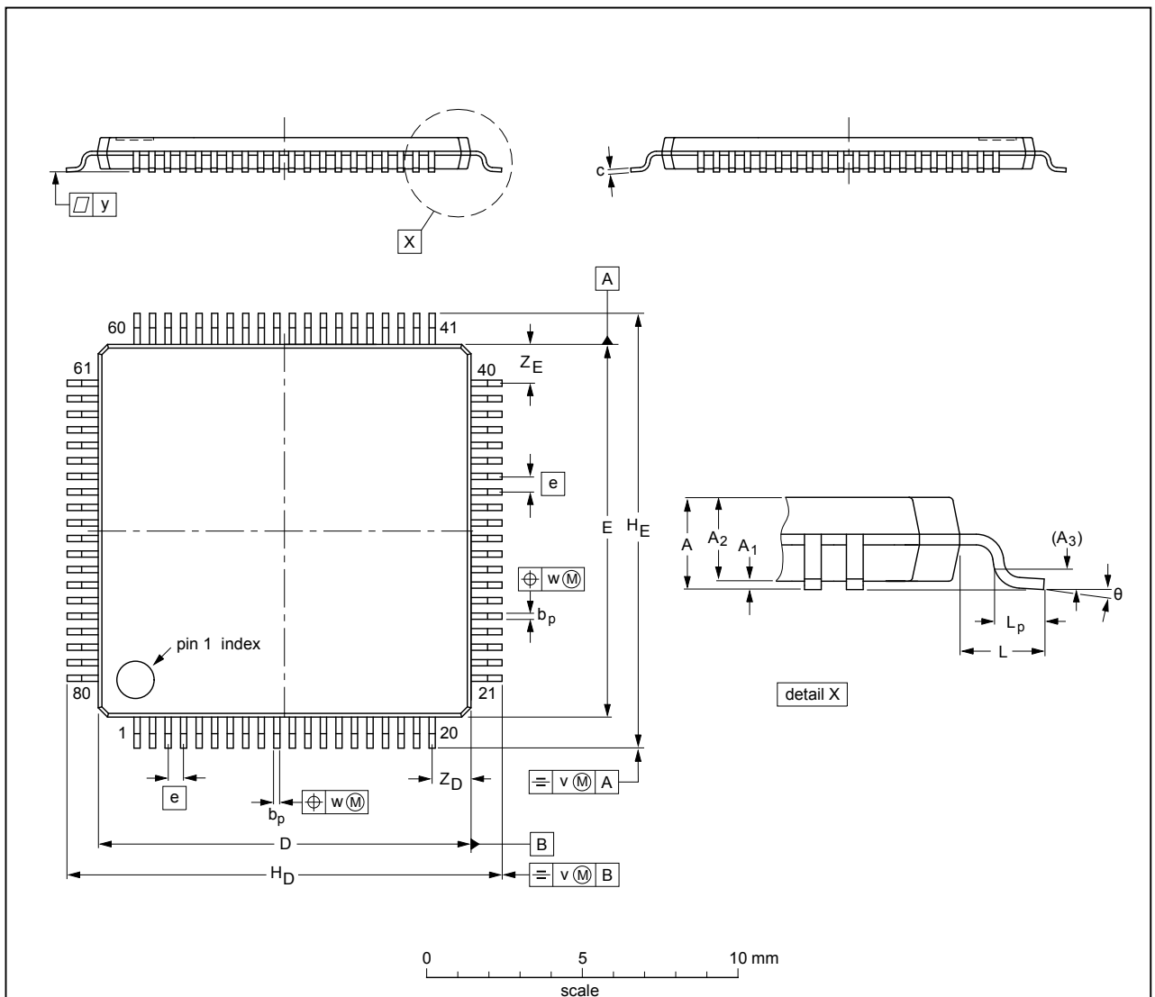
TQFP80: plastic thin quad flat package; 80 leads; body 12 x 12 x 1 mm
