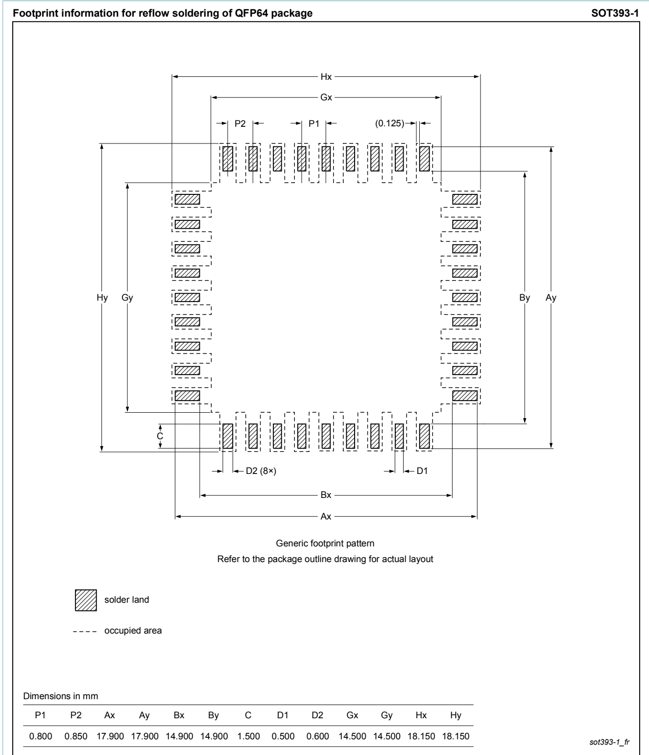
Fig. 2. Reflow soldering footprint for QFP64 (SOT393-1)
