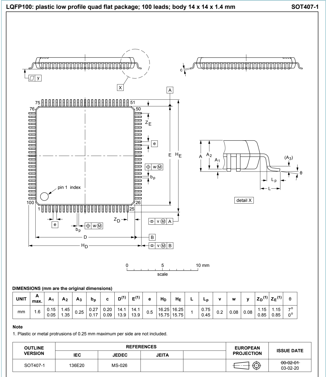
Figure 1. Package outline LQFP100 (SOT407-1)
