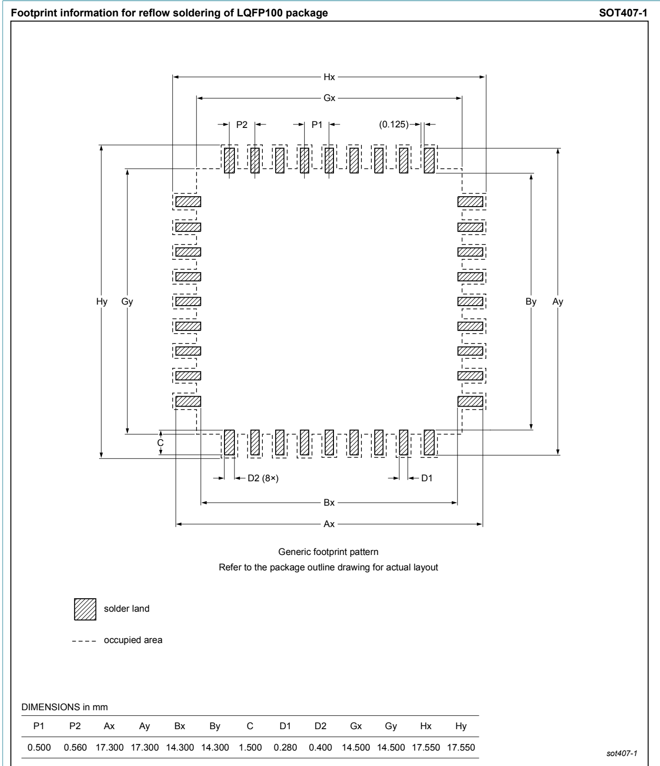
Figure 2. Reflow soldering footprint for LQFP100 (SOT407-1)
