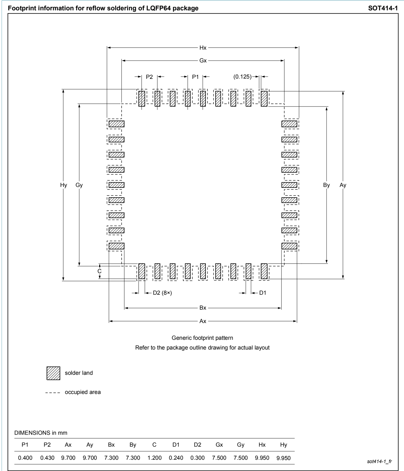
Fig. 2. Reflow soldering footprint for LQFP64 (SOT414-1)
