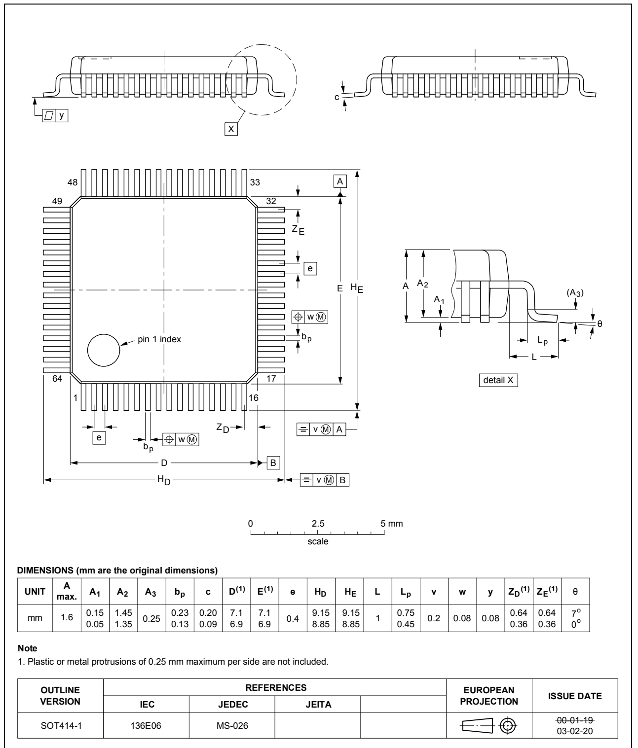
Fig. 1. Package outline LQFP64 (SOT414-1)
