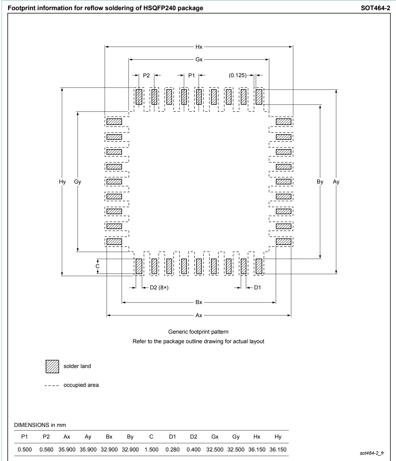
Fig. 2. Reflow soldering footprint for HSQFP240 (SOT464-2)
