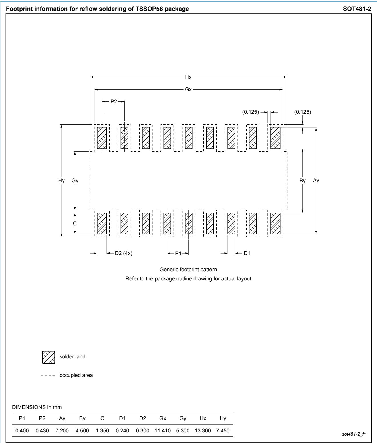
Fig. 2. Reflow soldering footprint for TSSOP56 (SOT481-2)
