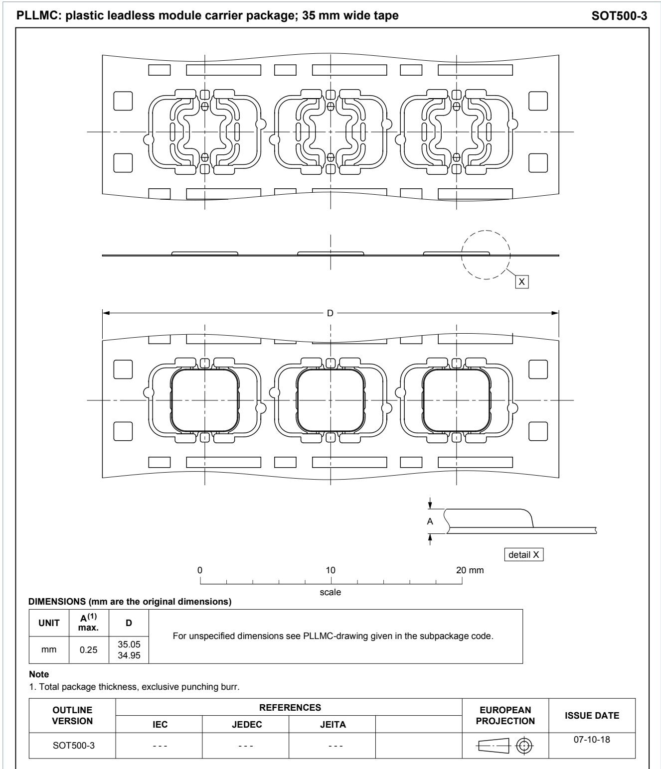
Fig. 1. Package outline PLLMC (SOT500-3)
