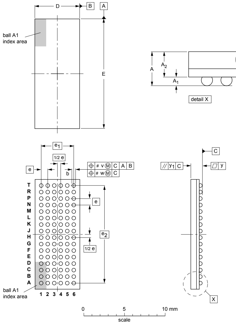
LFBGA96: plastic low profile fine-pitch ball grid array package; 96 balls; body 13.5 x 5.5 x 1.05 mm SOT536-1
