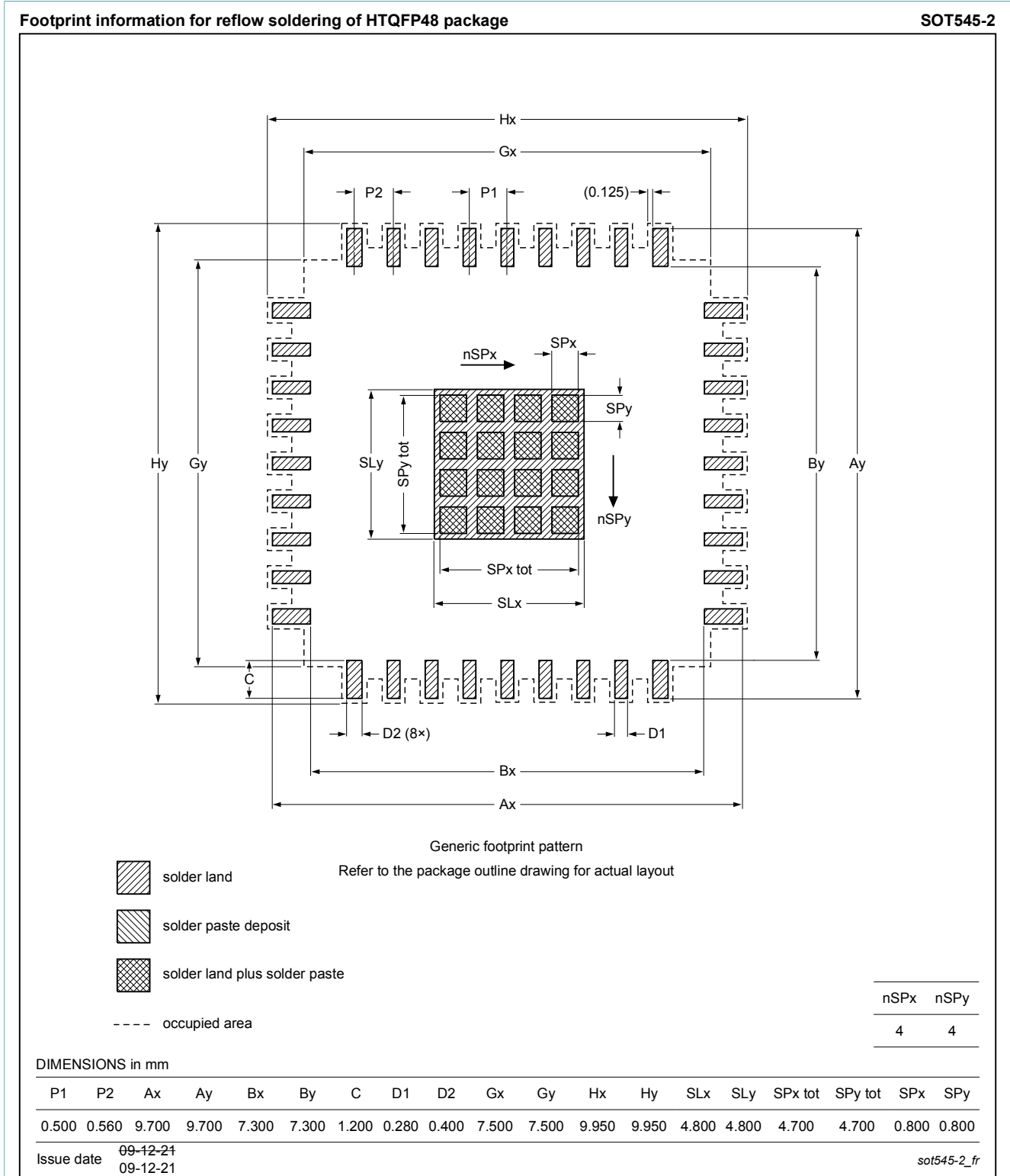
Fig. 2. Reflow soldering footprint for HTQFP48 (SOT545-2)
