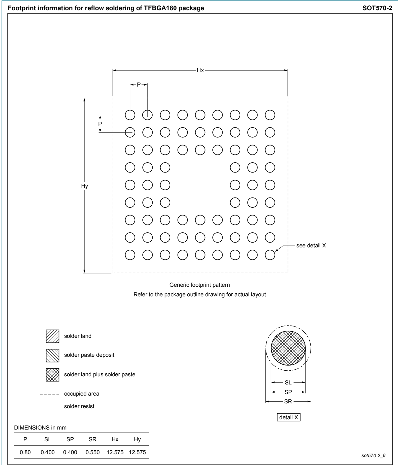
Fig. 2. Reflow soldering footprint for TFBGA180 (SOT570-2)
