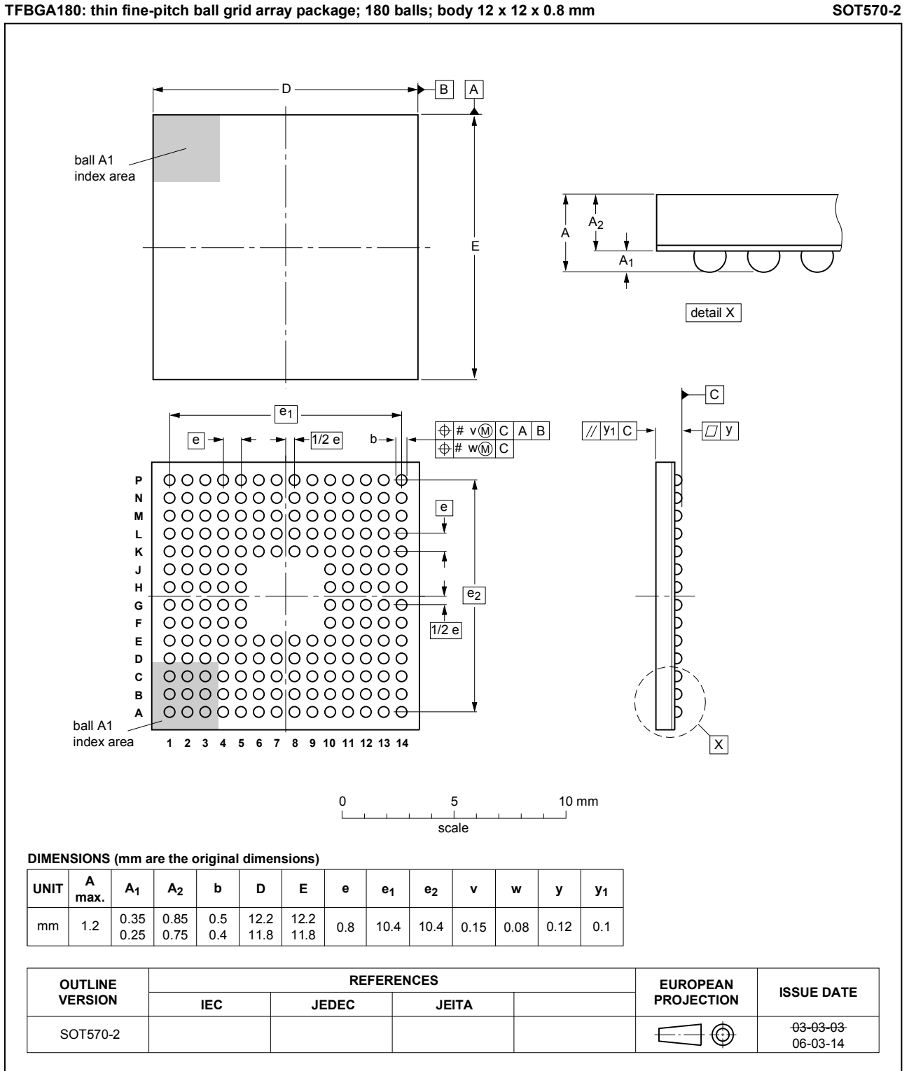
Fig. 1. Package outline TFBGA180 (SOT570-2)
