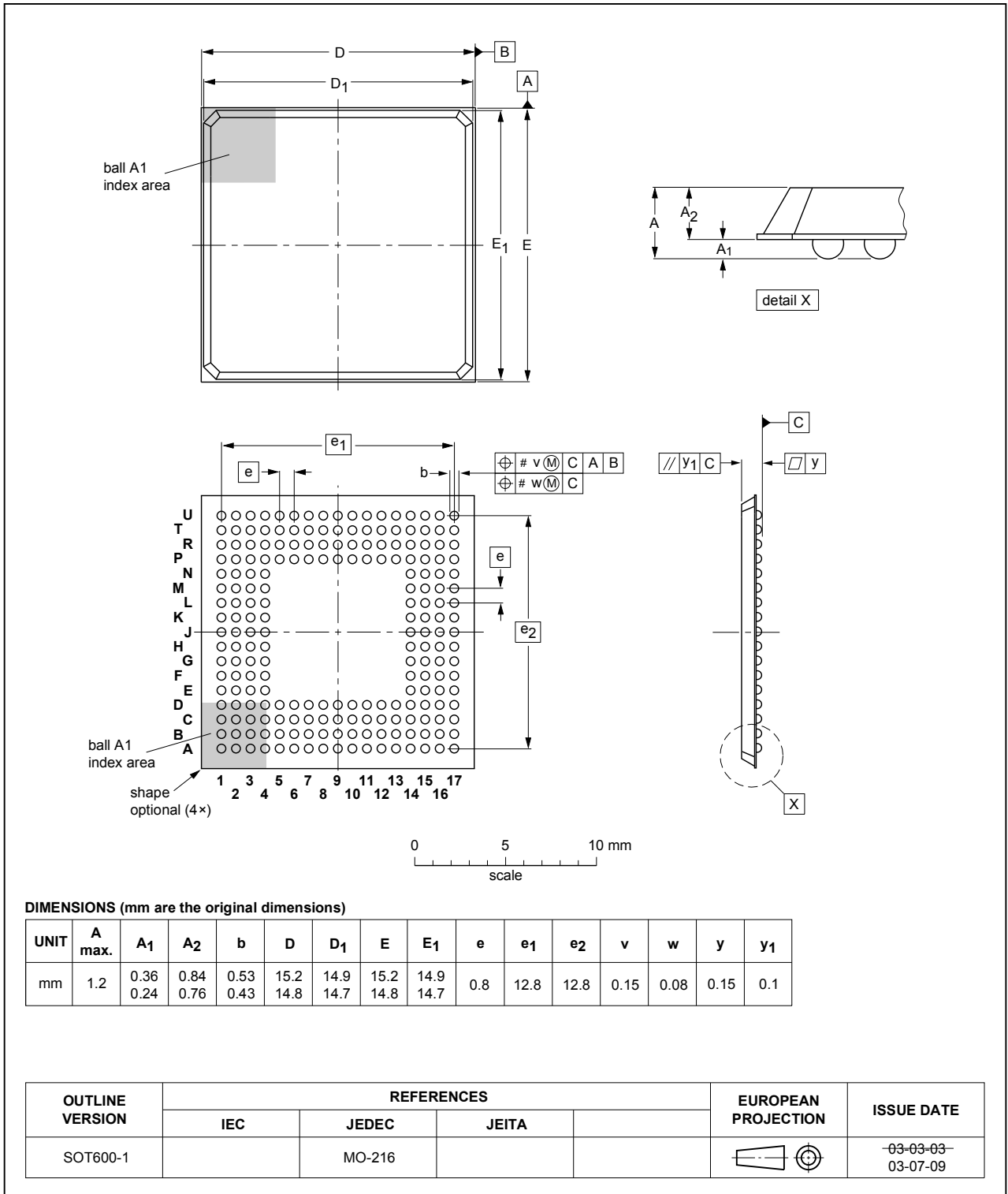
Fig. 1. Package outline TFBGA208 (SOT600-1)
