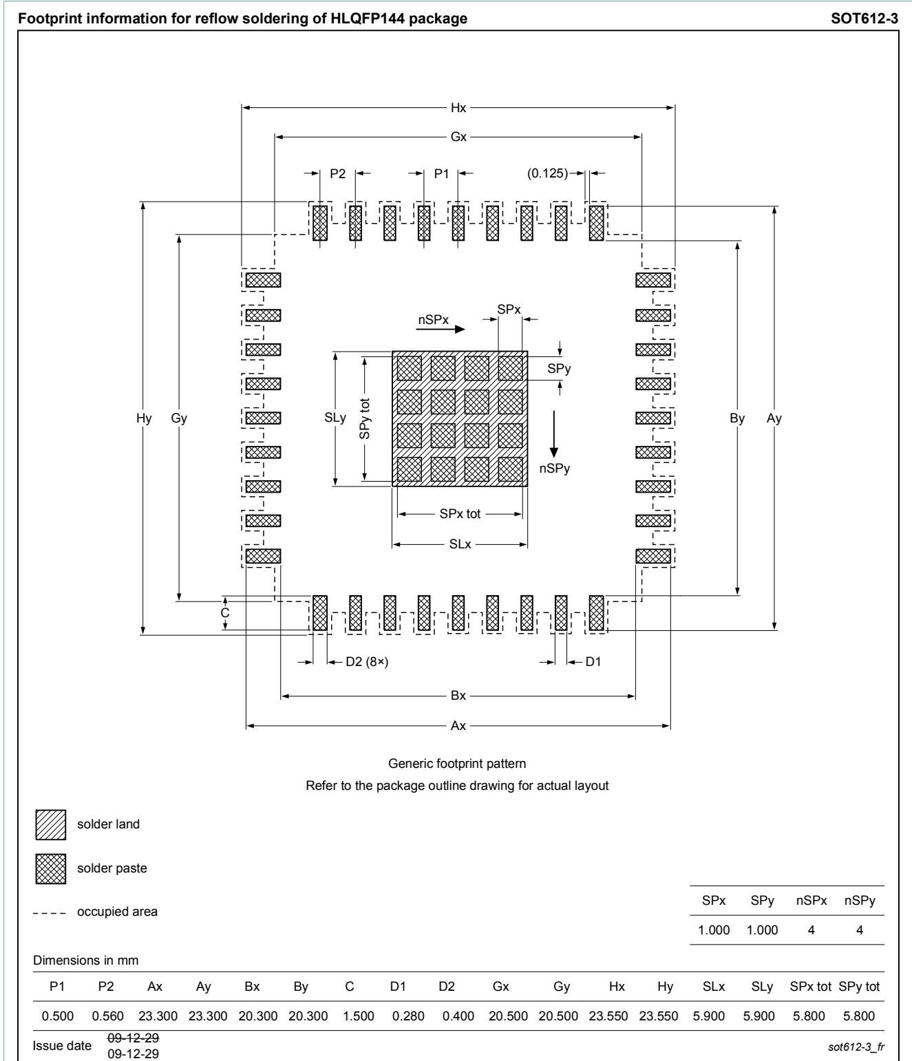
Fig. 2. Reflow soldering footprint for HLQFP144 (SOT612-3)
