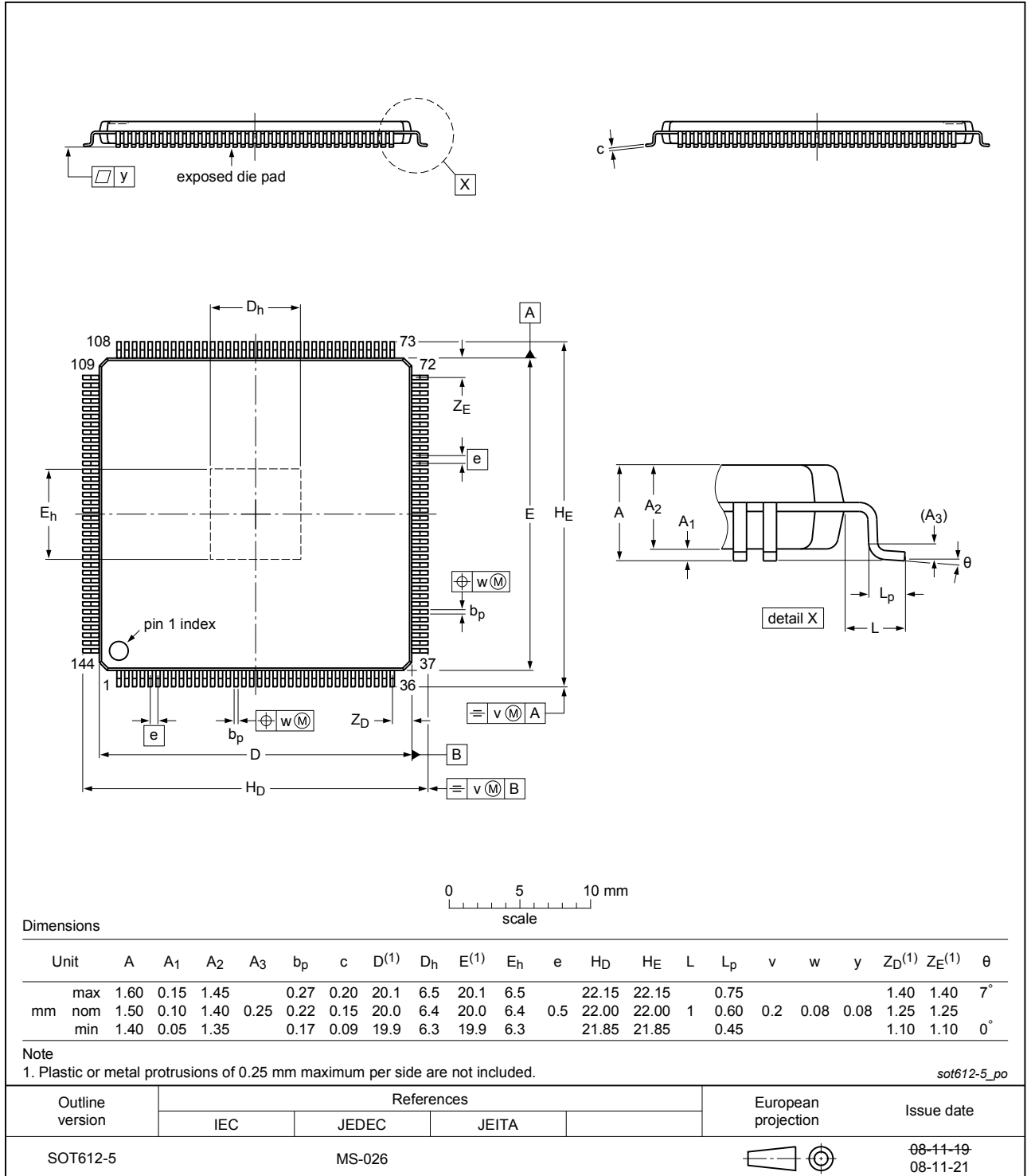
Fig. 1. Package outline HLQFP144 (SOT612-5)
