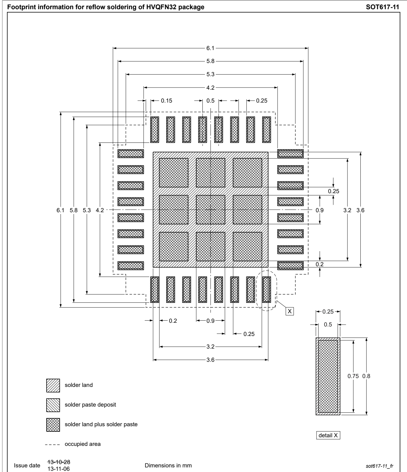
Figure 2. Reflow soldering footprint for HVQFN32 (SOT617-11)
