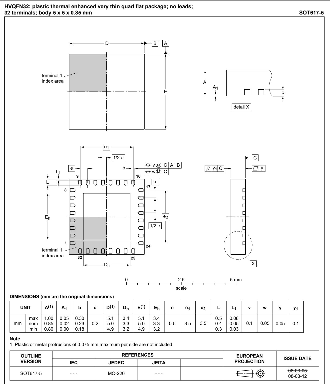
Figure 1. Package outline HVQFN32 (SOT617-5)
