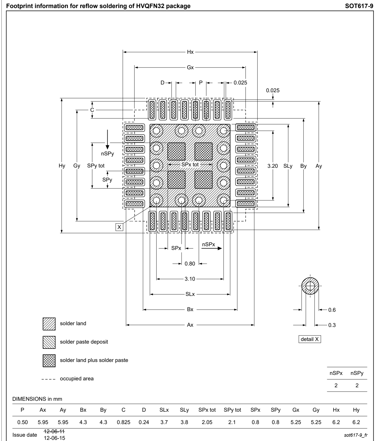
Figure 2. Reflow soldering footprint for HVQFN32 (SOT617-9)
