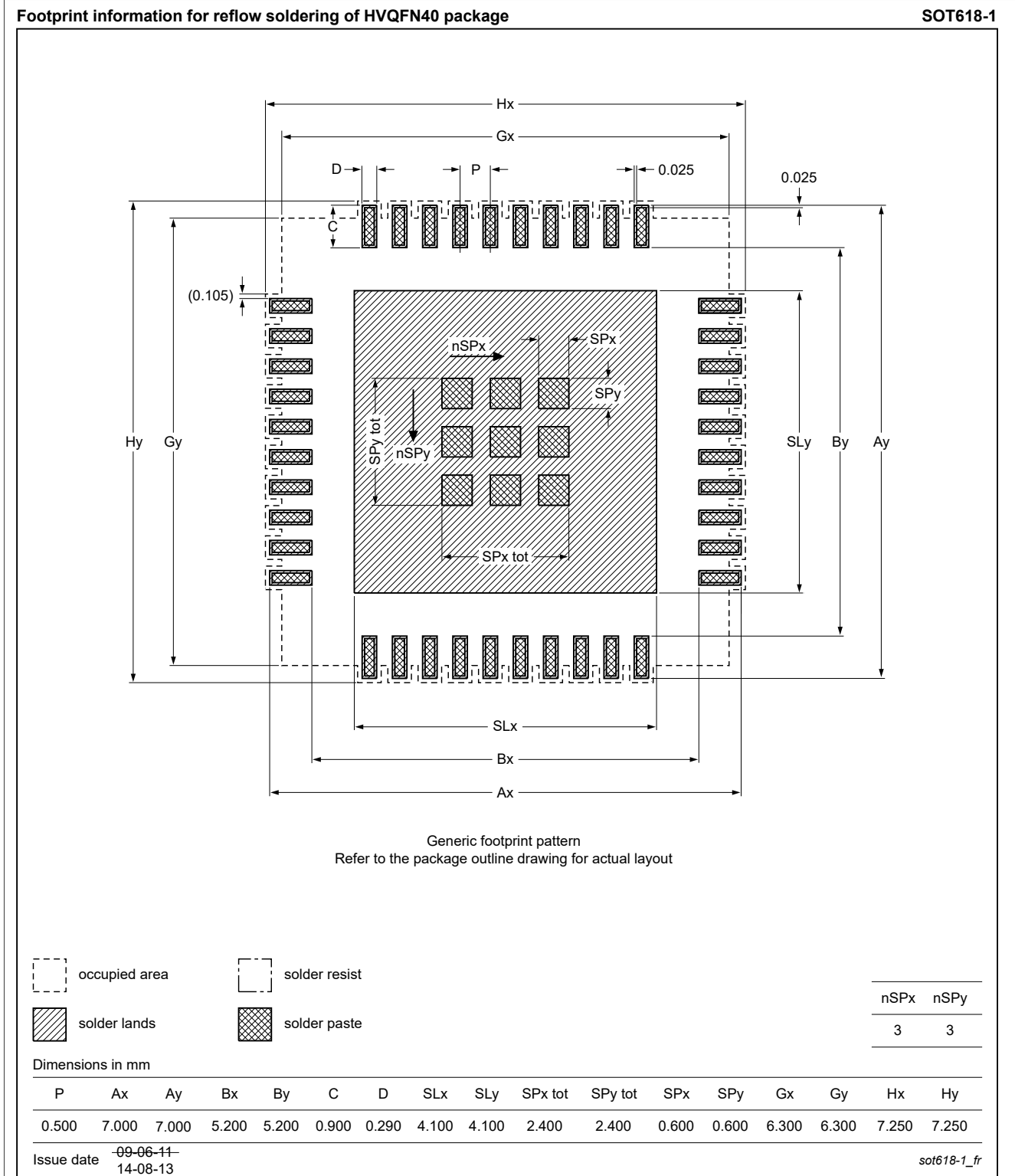
Figure 2. Reflow soldering footprint for HVQFN40 (SOT618-1)
