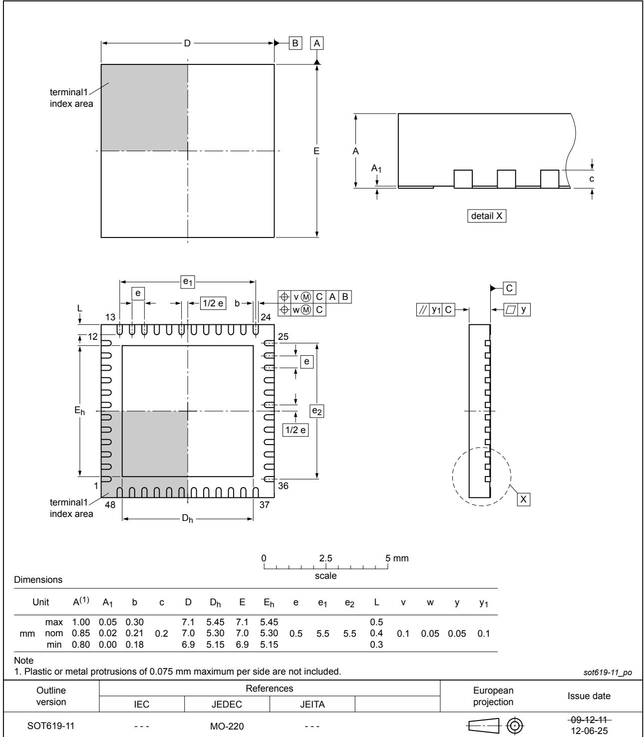
Fig. 1. Package outline HVQFN48 (SOT619-11)
