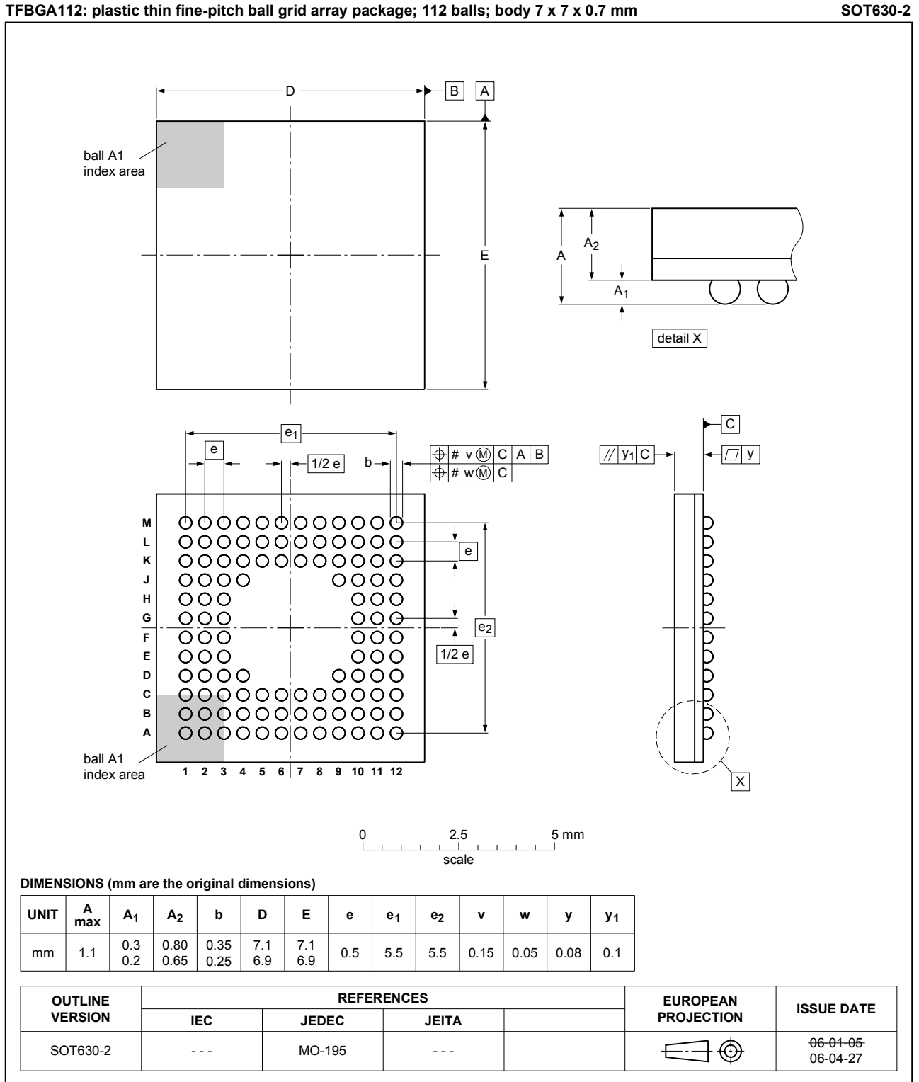
Fig. 1. Package outline TFBGA112 (SOT630-2)
