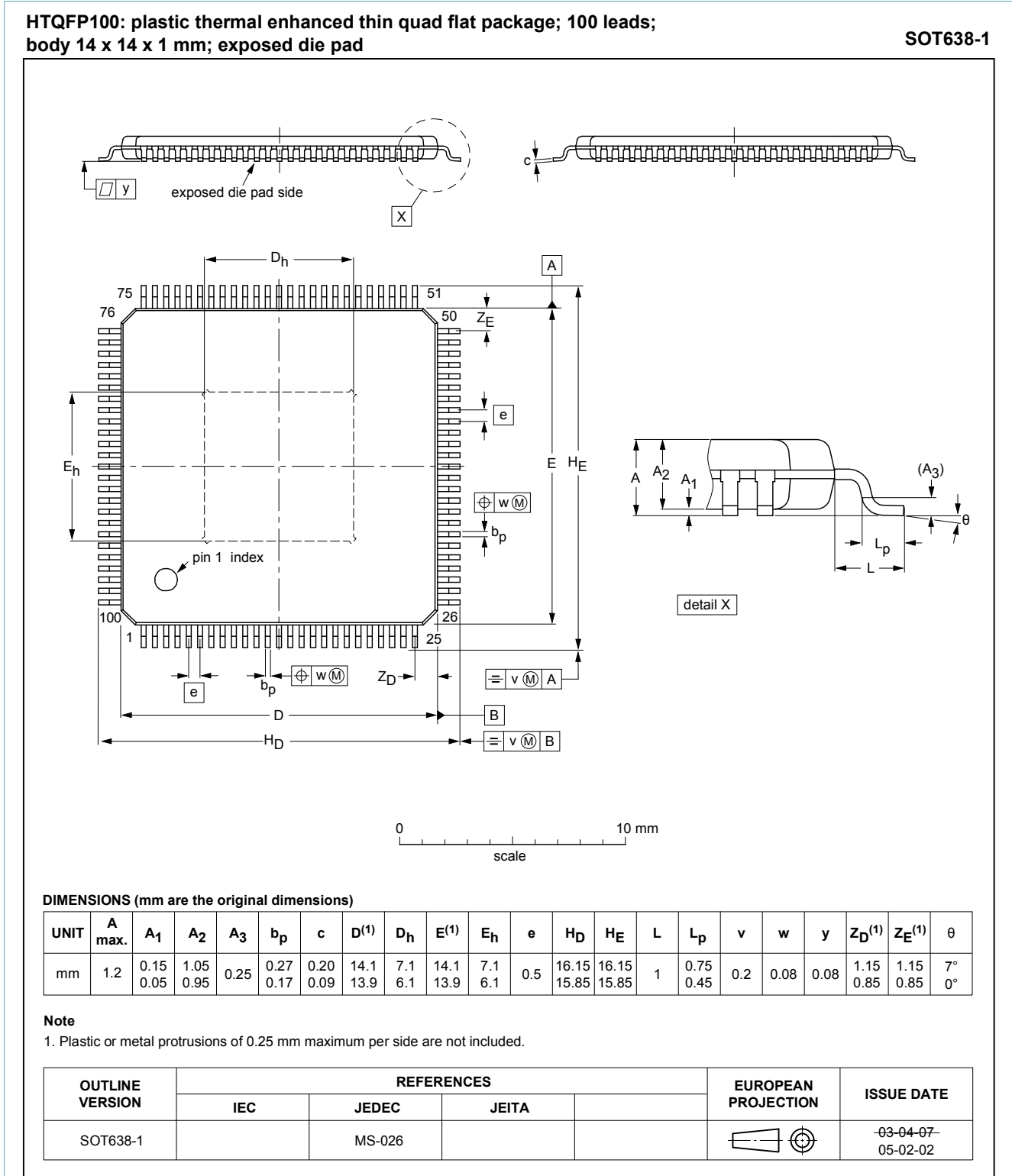
Fig. 1. Package outline HTQFP100 (SOT638-1)
