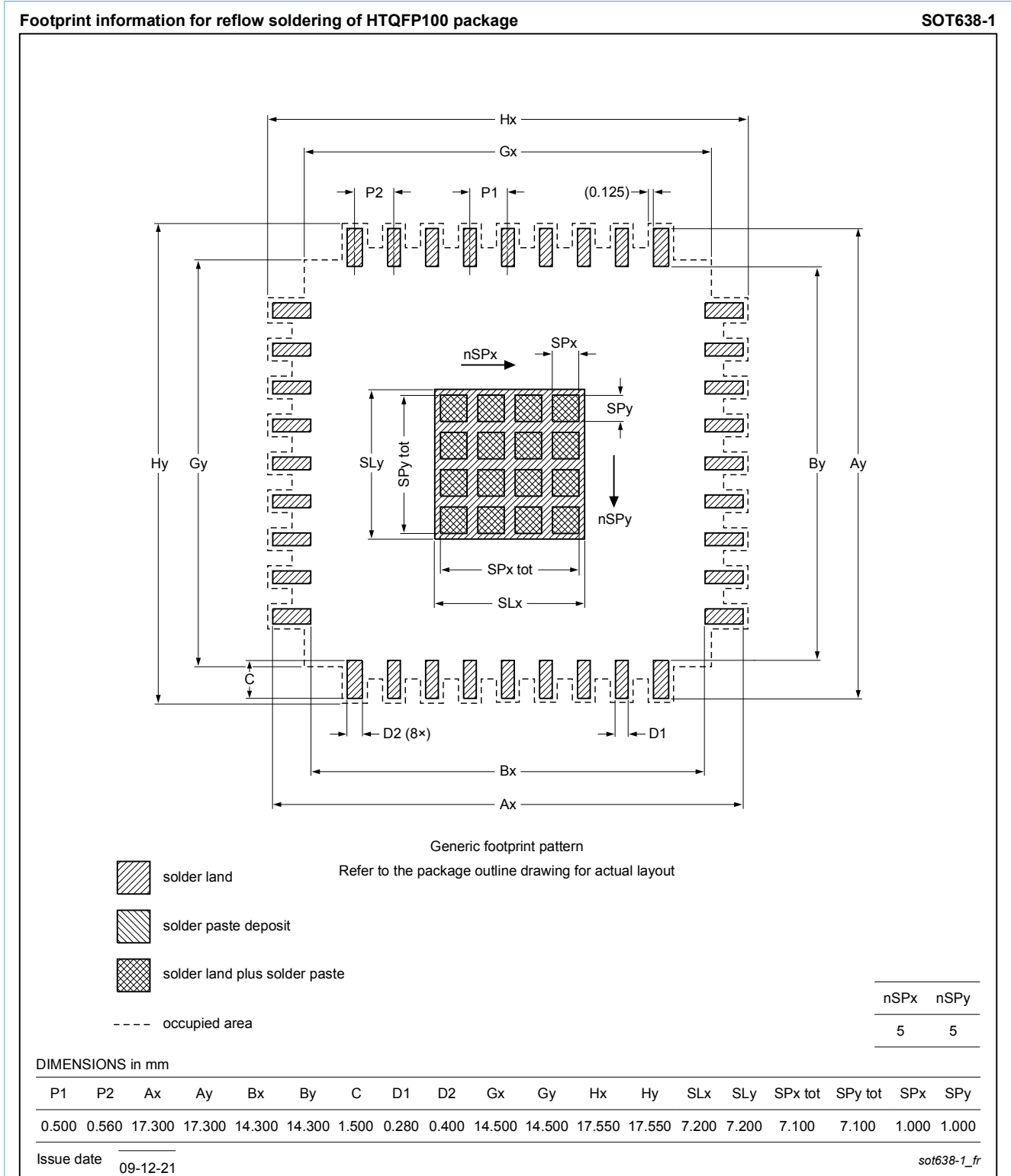
Fig. 2. Reflow soldering footprint for HTQFP100 (SOT638-1)
