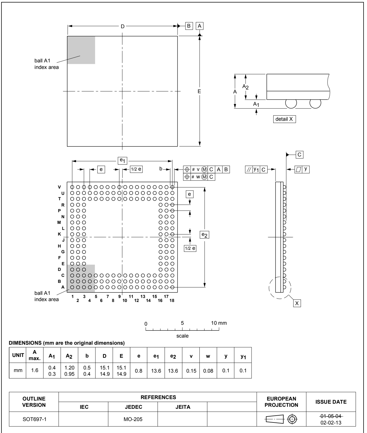
Fig. 1. Package outline LFBGA180 (SOT697-1)
