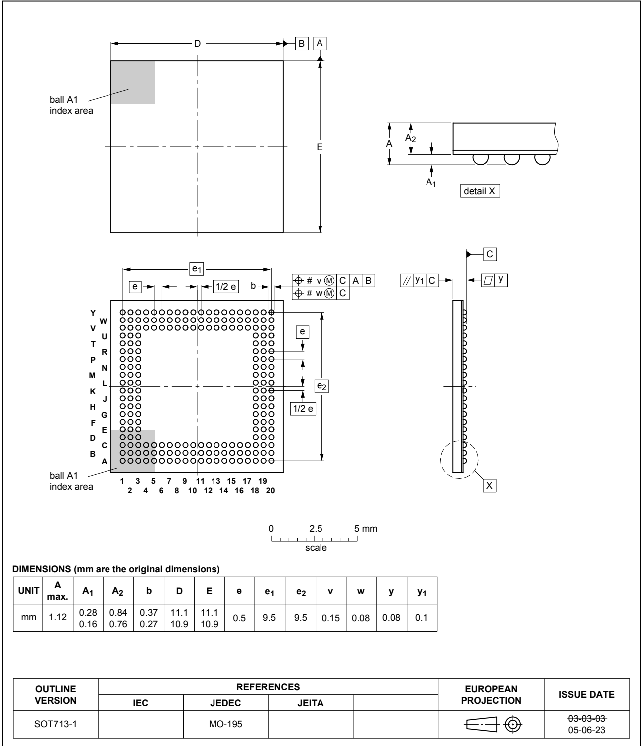
Fig. 1. Package outline TFBGA204 (SOT713-1)
