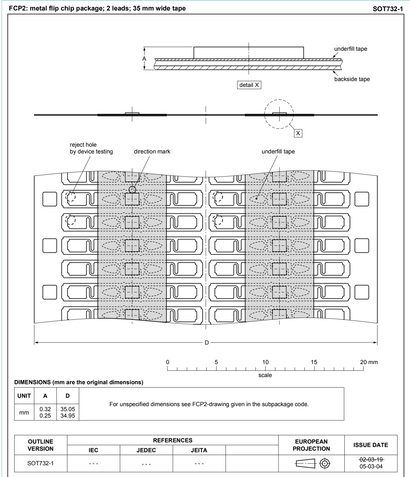
Fig. 1. Package outline FCP2 (SOT732-1)
