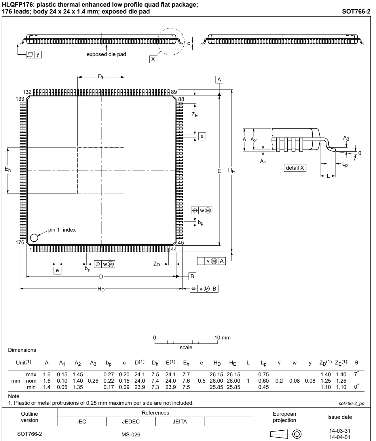
Fig. 1. Package outline HLQFP176 (SOT766-2)
