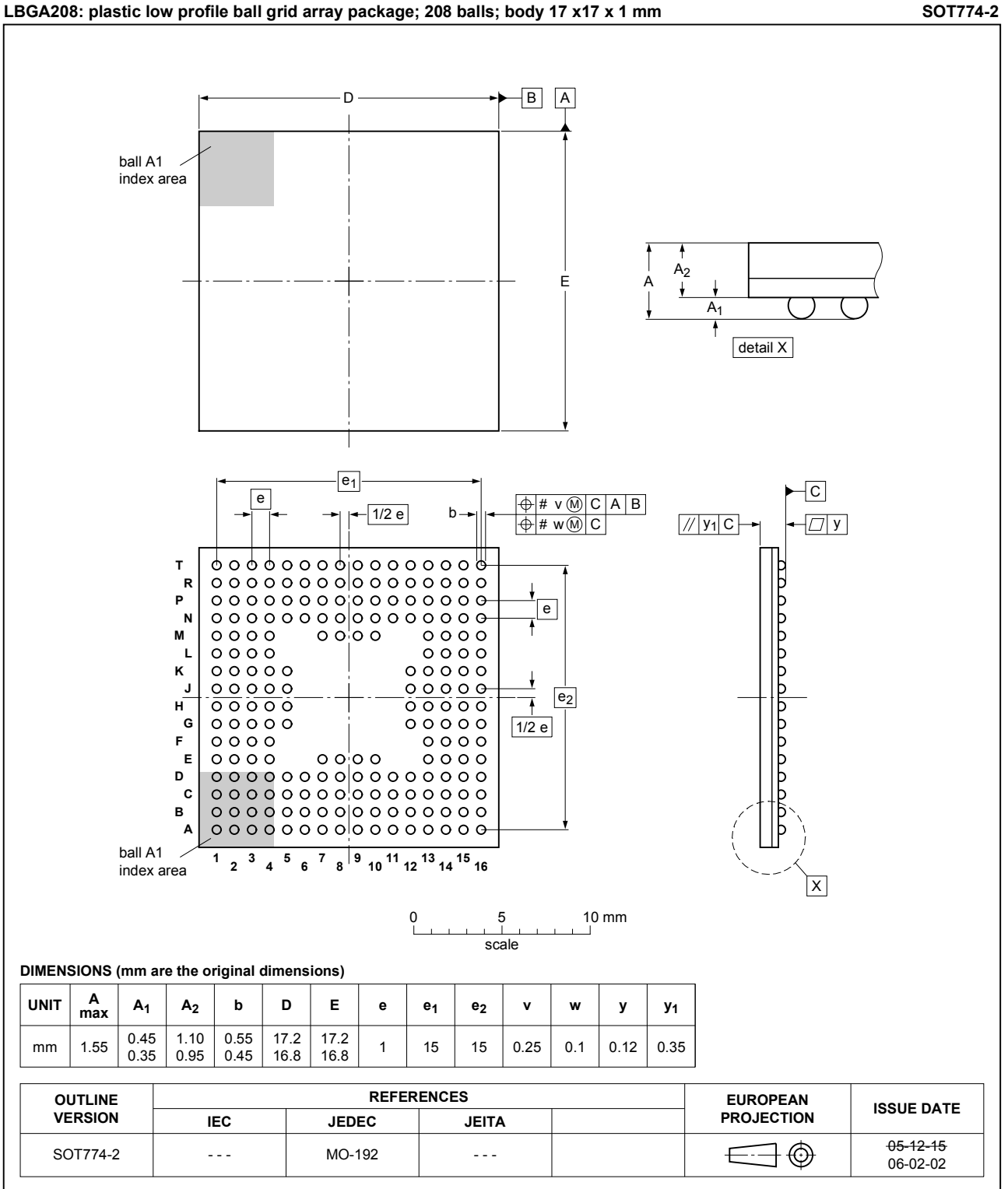
Fig. 1. Package outline LPGA208 (SOT774-2)
