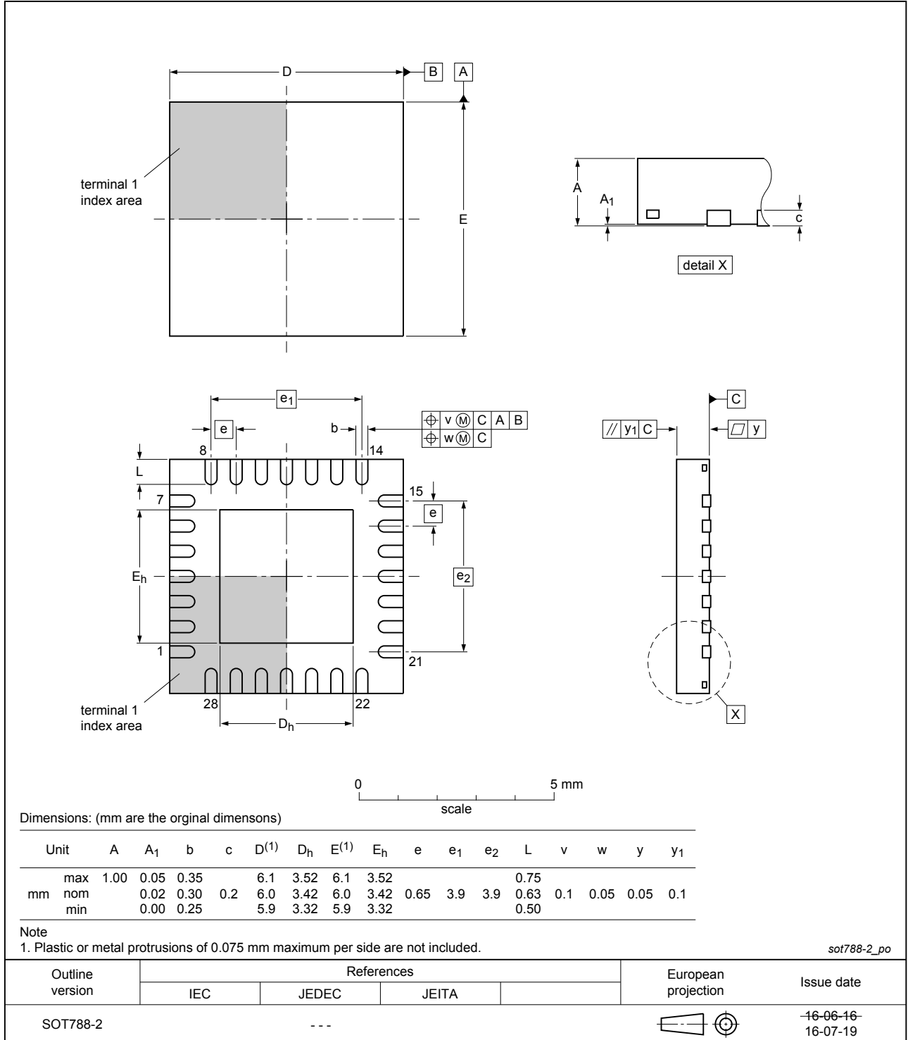
Fig. 1. Package outline HVQFN (SOT788-2)
