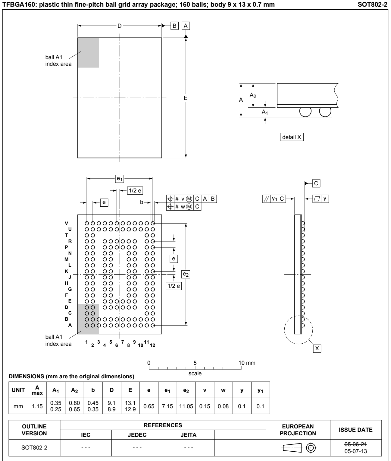
Fig. 1. Package outline TFBGA160 (SOT802-2)
