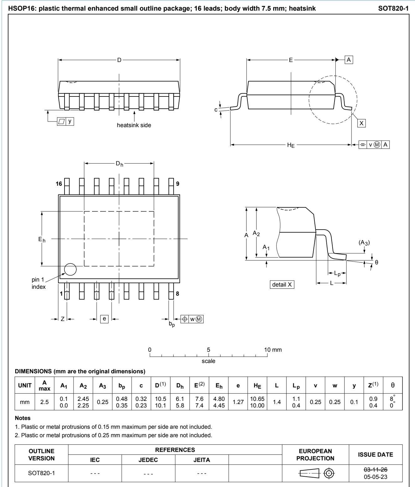
Fig. 1. Package outline HSOP16 (SOT820-1)
