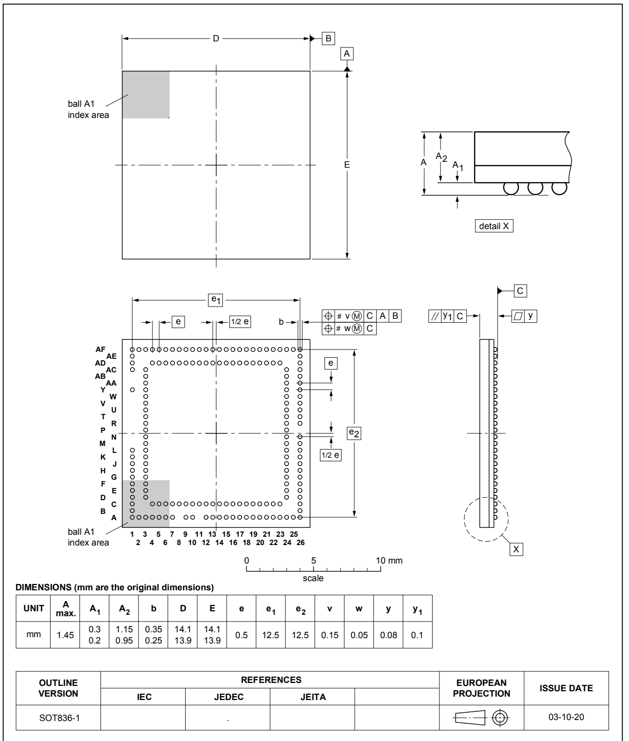
Fig. 1. Package outline LFBGA167 (SOT836-1)
