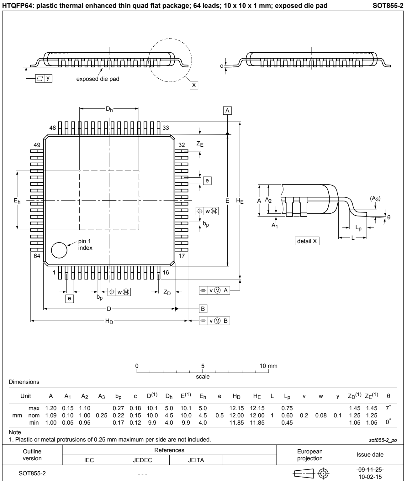
Fig. 1. Package outline HTQFP64 (SOT855-2)
